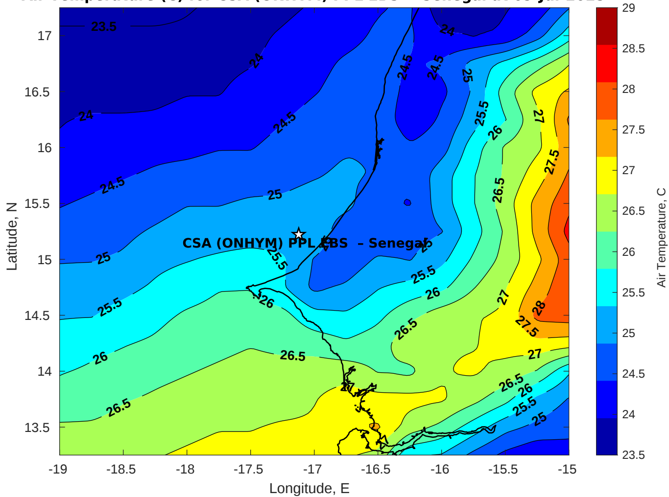
Air Temperature (C) for CSA (ONHYM) PPL EBS - Senegal at 09-Jul-2025
