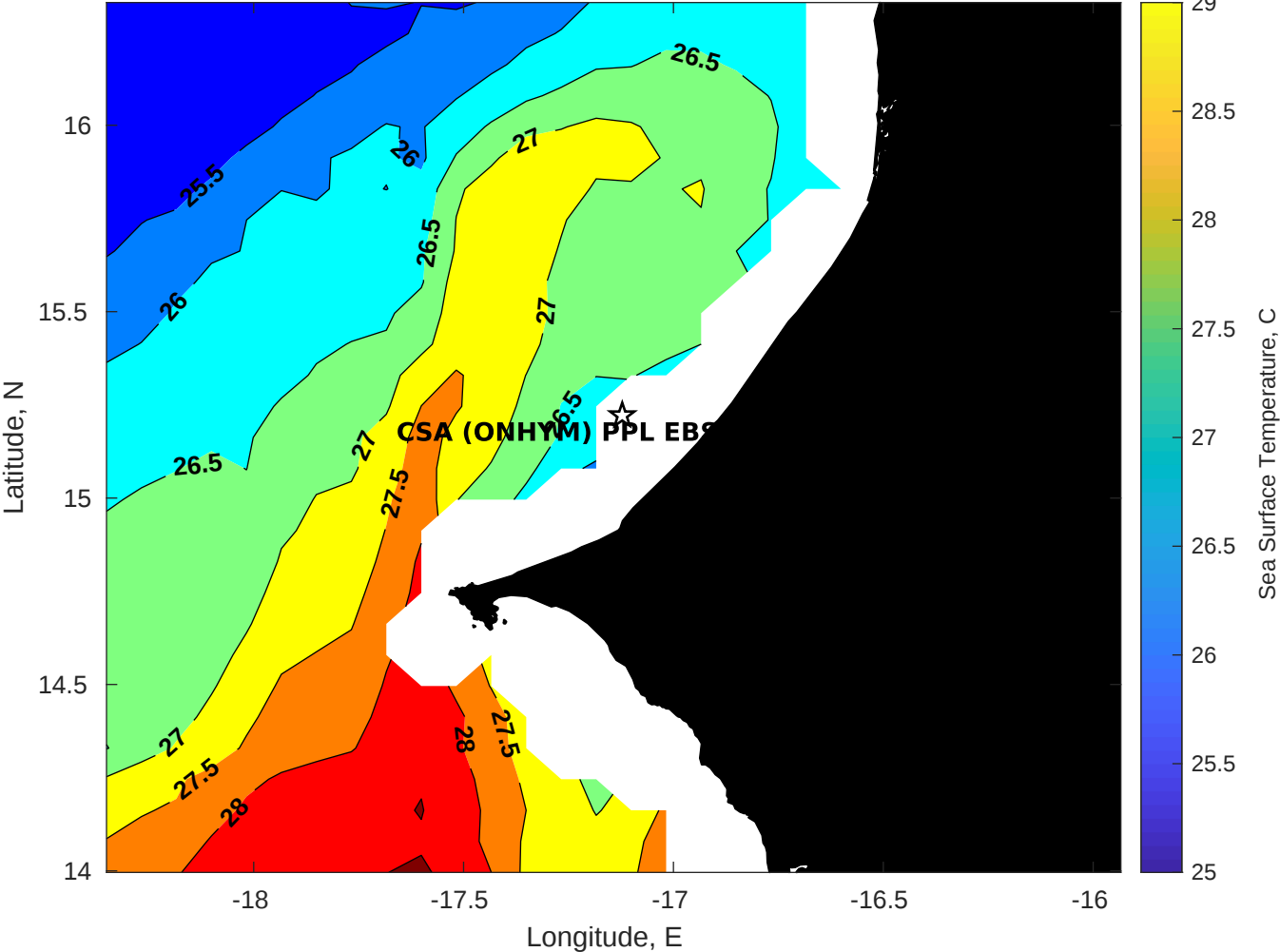
SST for CSA (ONHYM) PPL EBS - Senegal at 08-Jul-2025 00:00:00
