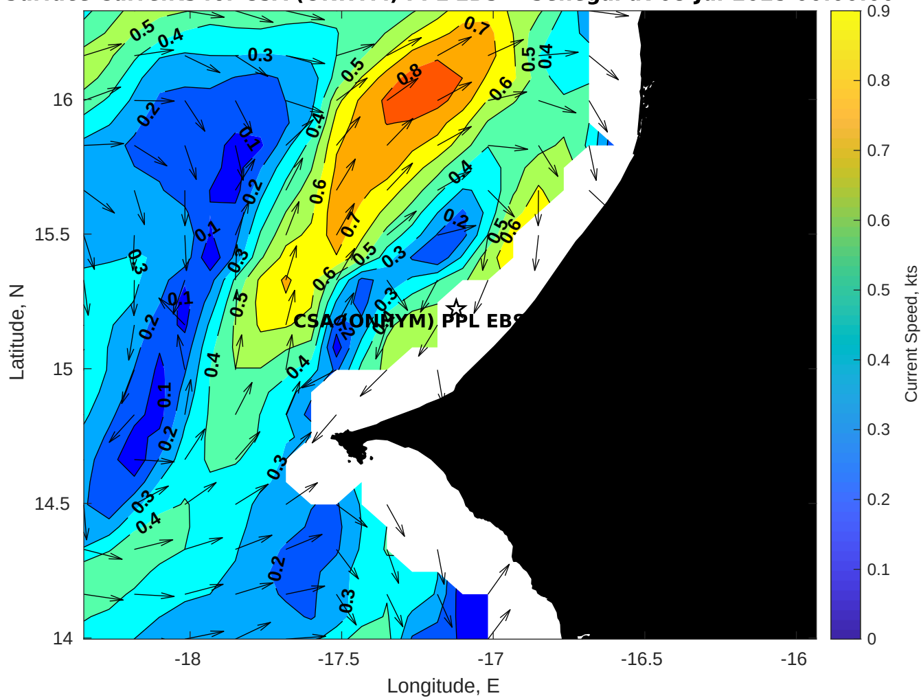
Surface Currents for CSA (ONHYM) PPL EBS - Senegal at 08-Jul-2025 00:00:00
