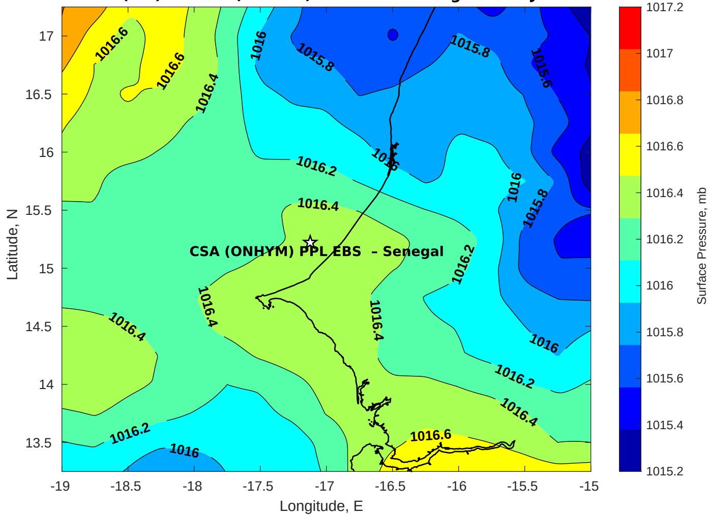
Surface Pressure (mb) for CSA (ONHYM) PPL EBS - Senegal at 11-Jul-2025 00:00:00
