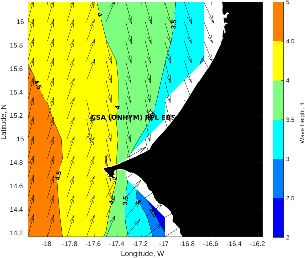
Wave Height (ft) for CSA (ONHYM) PPL EBS - Senegal at 09-Jul-2025 09:00:00
