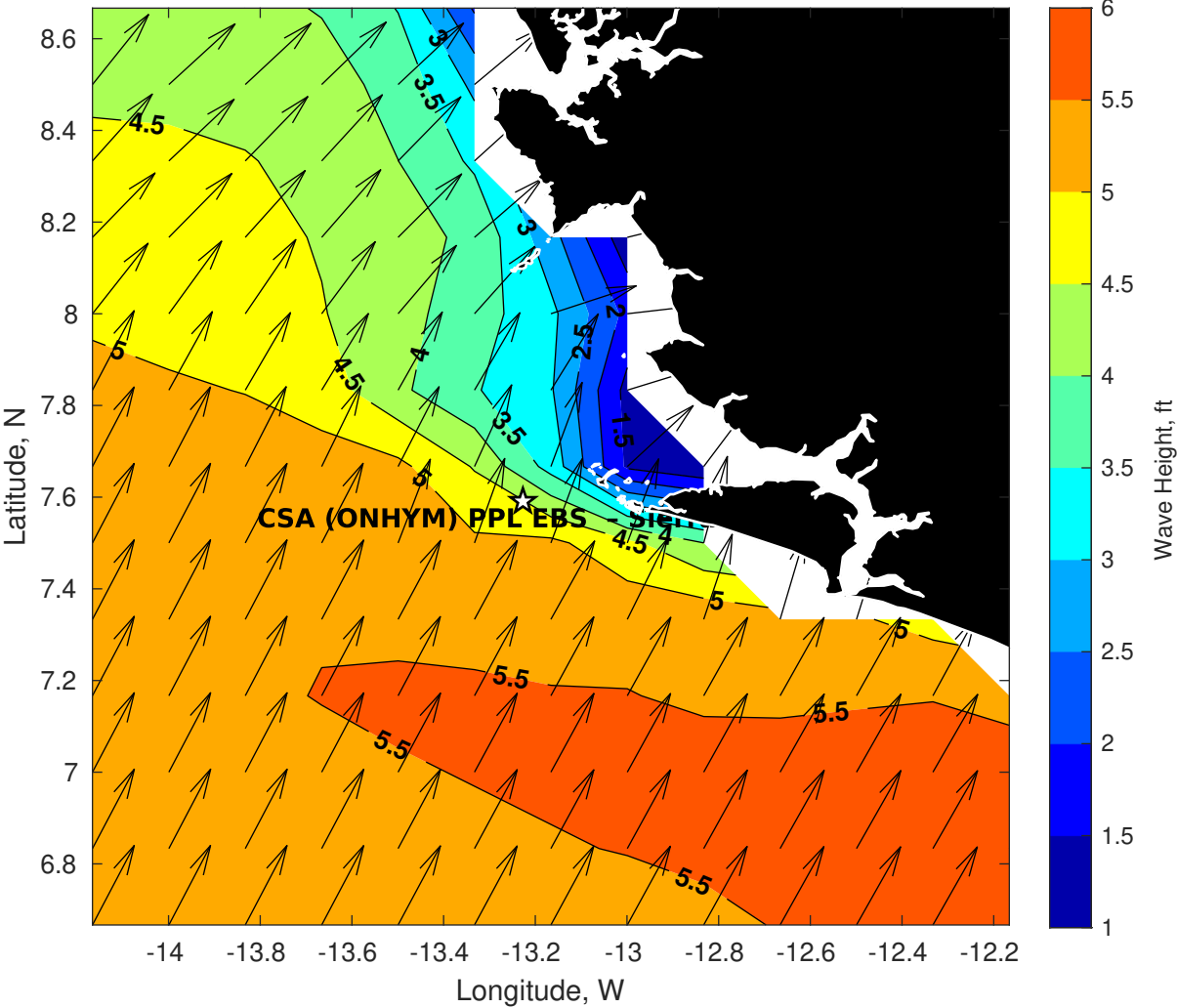
Wave Height (ft) for CSA (ONHYM) PPL EBS - Sierra Leone at 09-Jul-2025 09:00:00
