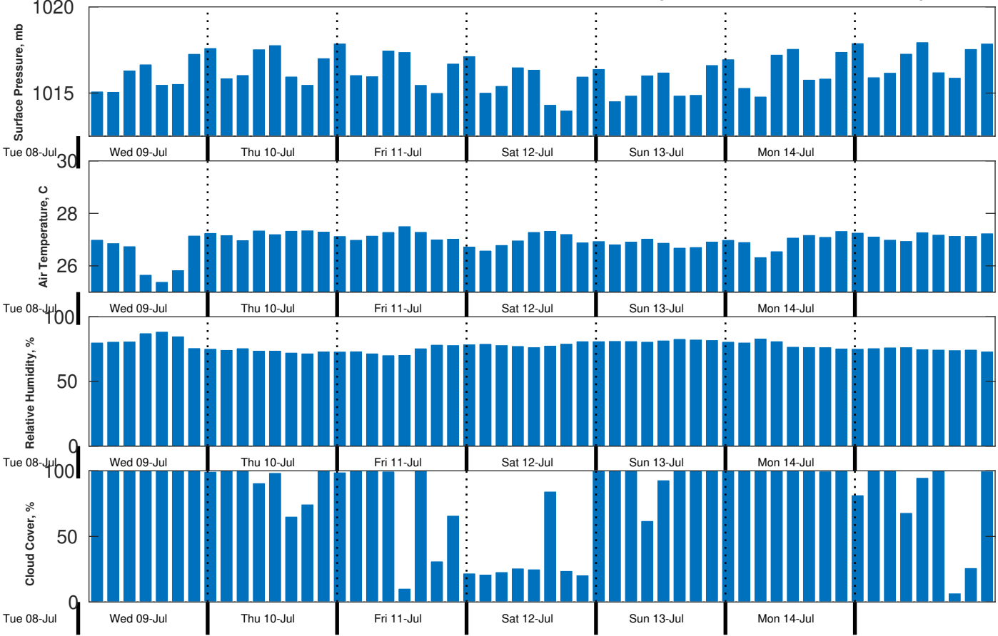
Met Forecast for CSA (ONHYM) PPL EBS - Sierra Leone from 09-Jul-2025 00:00:00 to 16-Jul-2025 00:00:00
