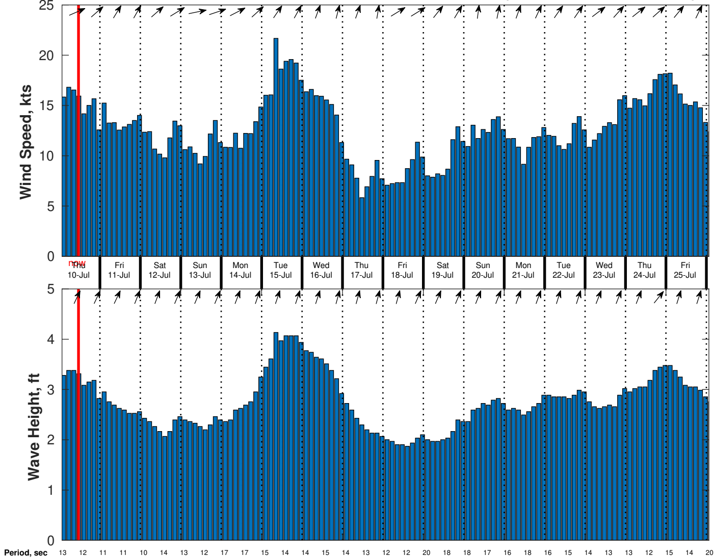
Wind & Wave Forecast for CSA (ONHYM) PPL EBS - Sierra Leone from 09-Jul-2025 01:00:00 to 25-Jul-2025 01:00:00
