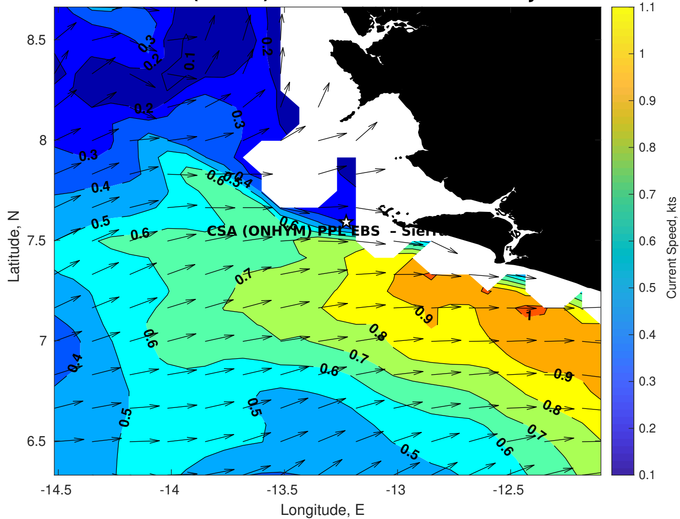
Surface Currents for CSA (ONHYM) PPL EBS - Sierra Leone at 08-Jul-2025 00:00:00
