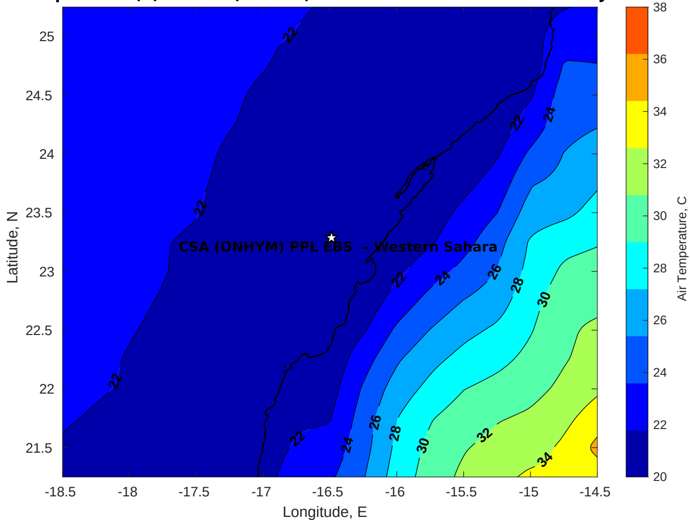
Air Temperature (C) for CSA (ONHYM) PPL EBS - Western Sahara at 09-Jul-2025
