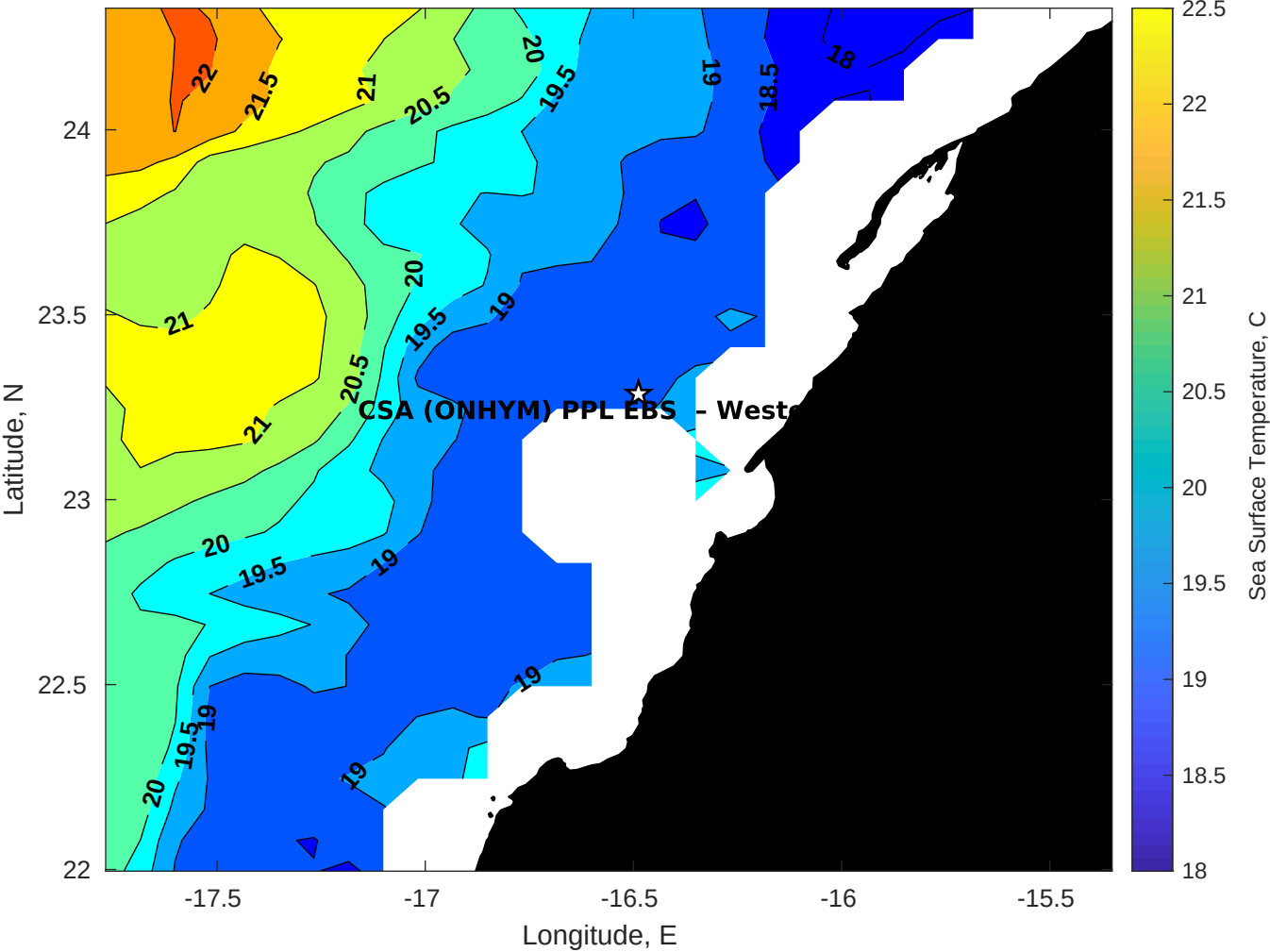
SST for CSA (ONHYM) PPL EBS - Western Sahara at 08-Jul-2025 00:00:00
