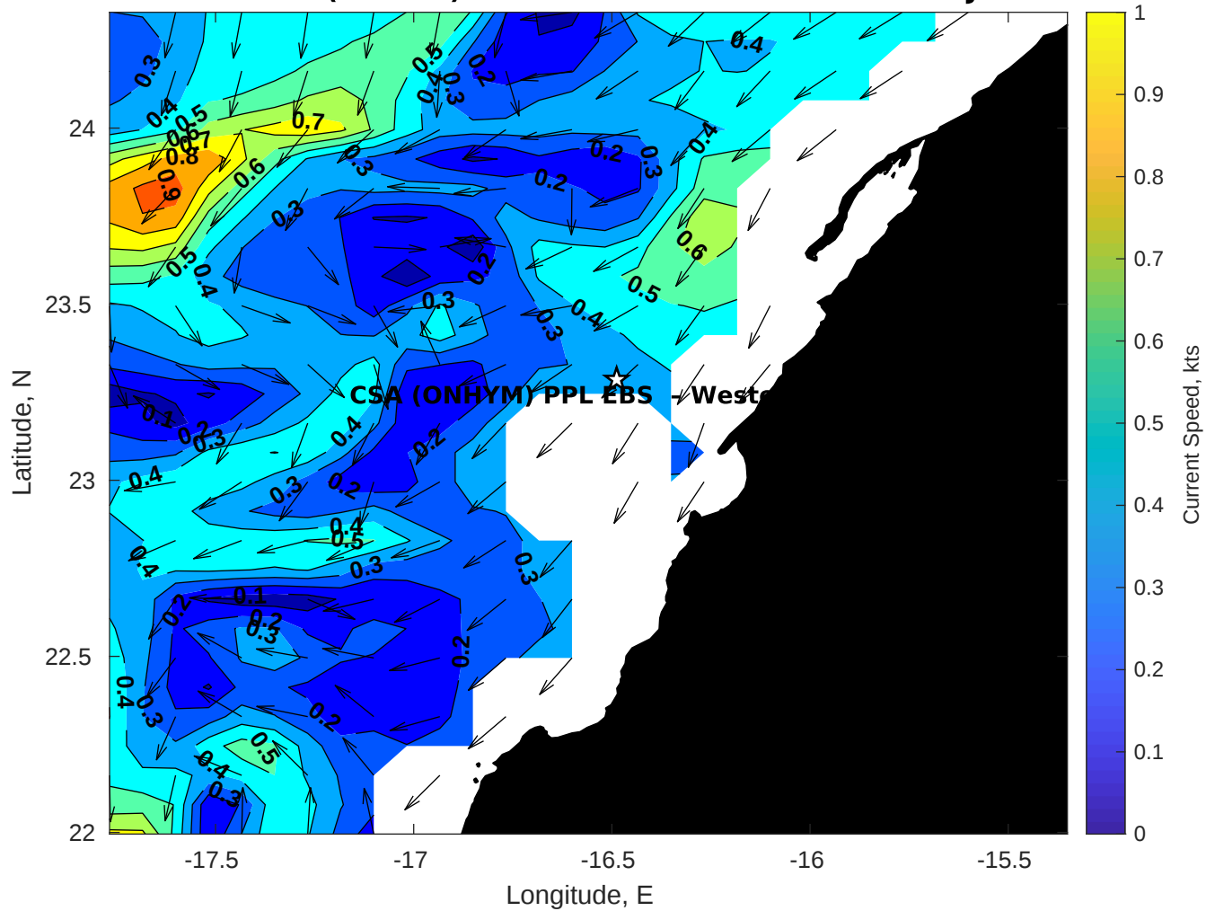
Surface Currents for CSA (ONHYM) PPL EBS - Western Sahara at 08-Jul-2025 00:00:00
