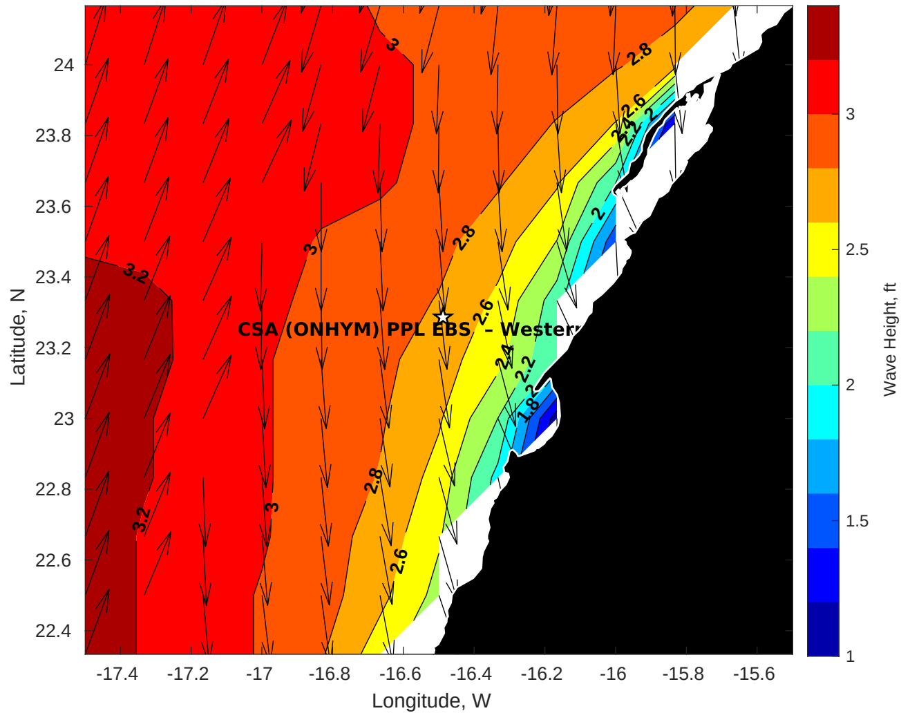
Wave Height (ft) for CSA (ONHYM) PPL EBS - Western Sahara at 09-Jul-2025 09:00:00
