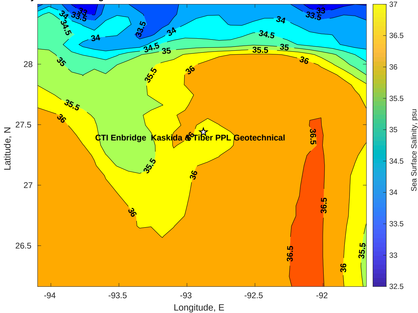
Surface Salinity for CTI Enbridge Kaskida & Tiber PPL Geotechnical at 08-Jul-2025 00:00:00
