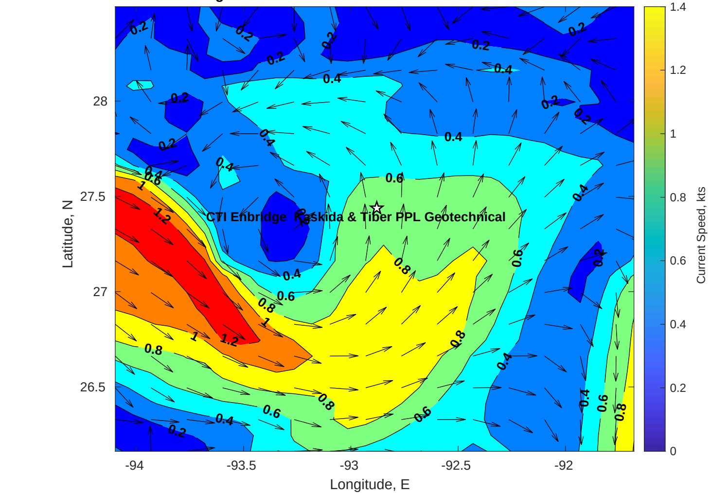
Surface Currents for CTI Enbridge Kaskida & Tiber PPL Geotechnical at 08-Jul-2025 00:00:00
