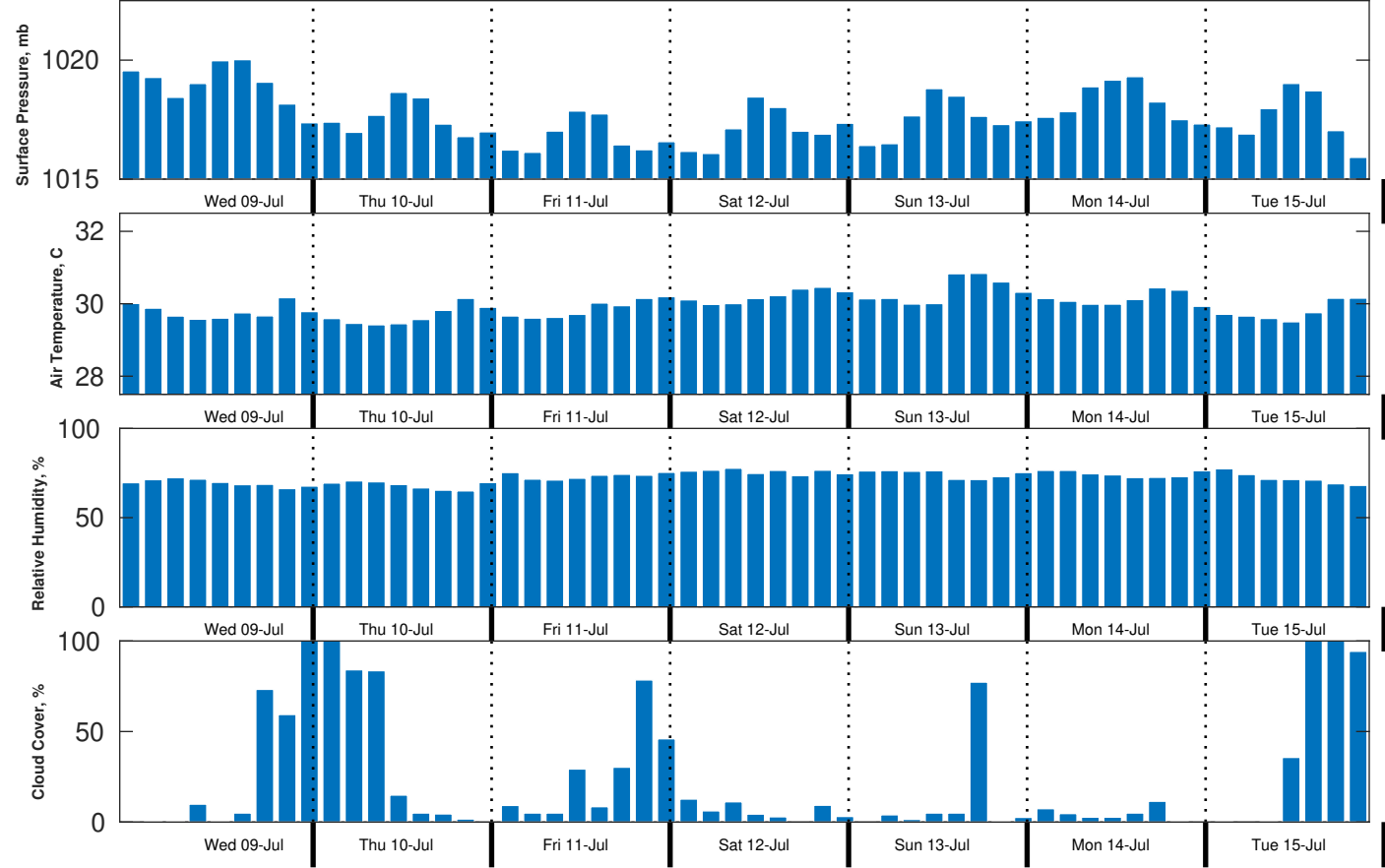
Met Forecast for CTI Enbridge Kaskida & Tiber PPL Geotechnical from 09-Jul-2025 00:00:00 to 16-Jul-2025 00:00:00
