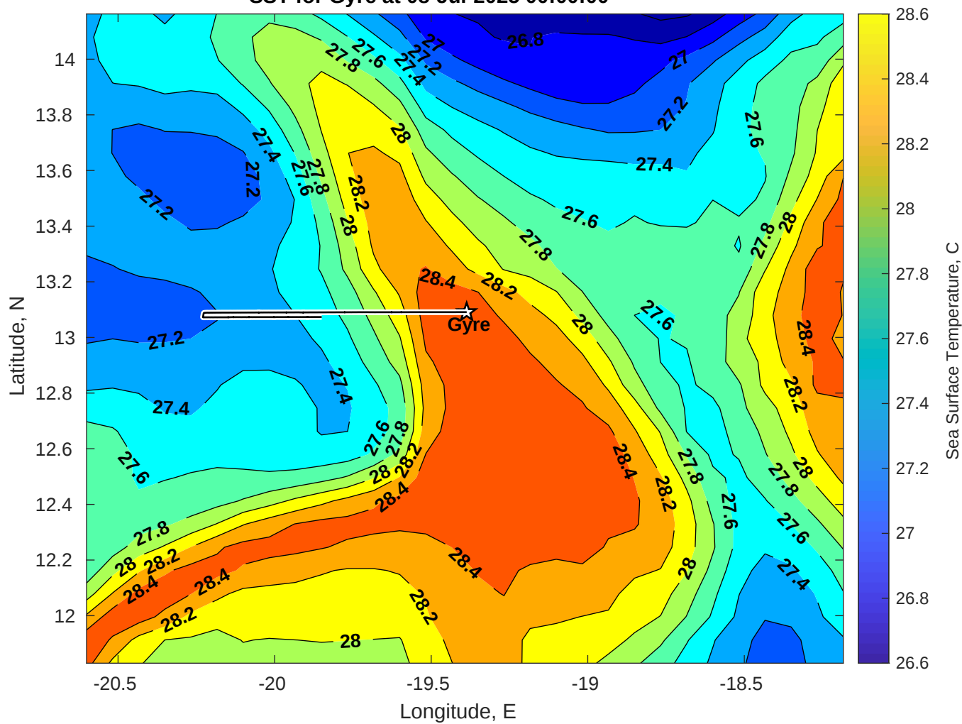
SST for Gyre at 08-Jul-2025 00:00:00
