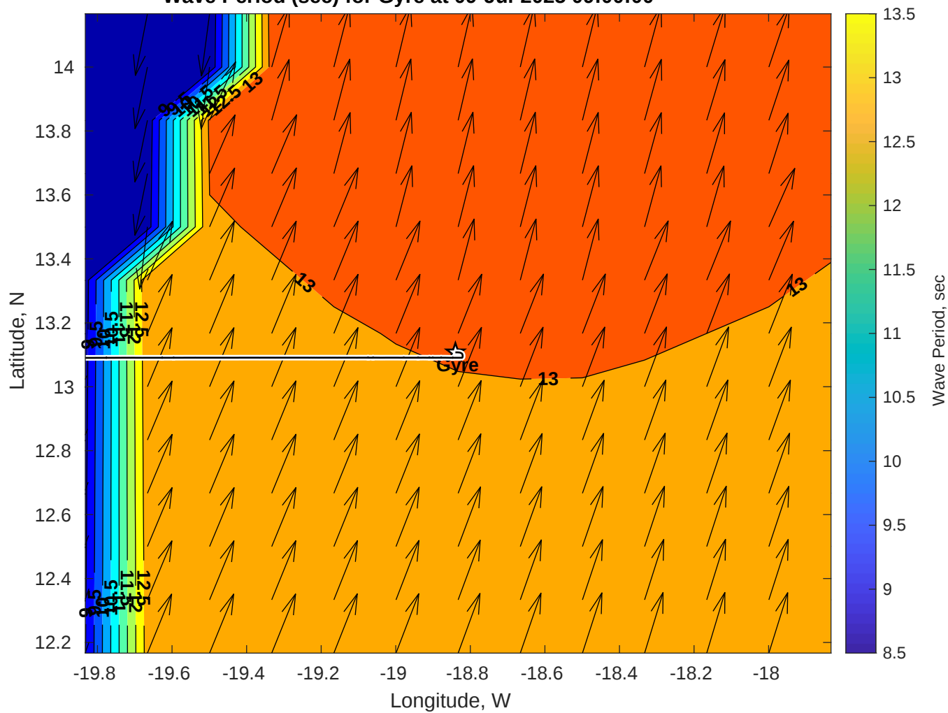
Wave Period (sec) for Gyre at 09-Jul-2025 09:00:00
