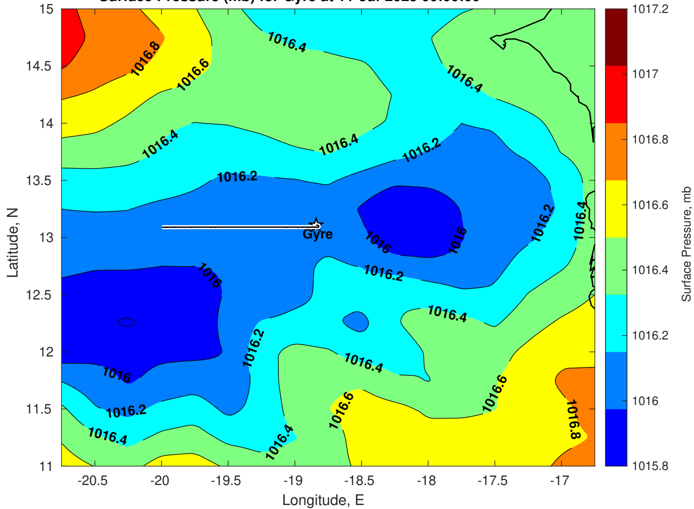
Surface Pressure (mb) for Gyre at 11-Jul-2025 00:00:00
