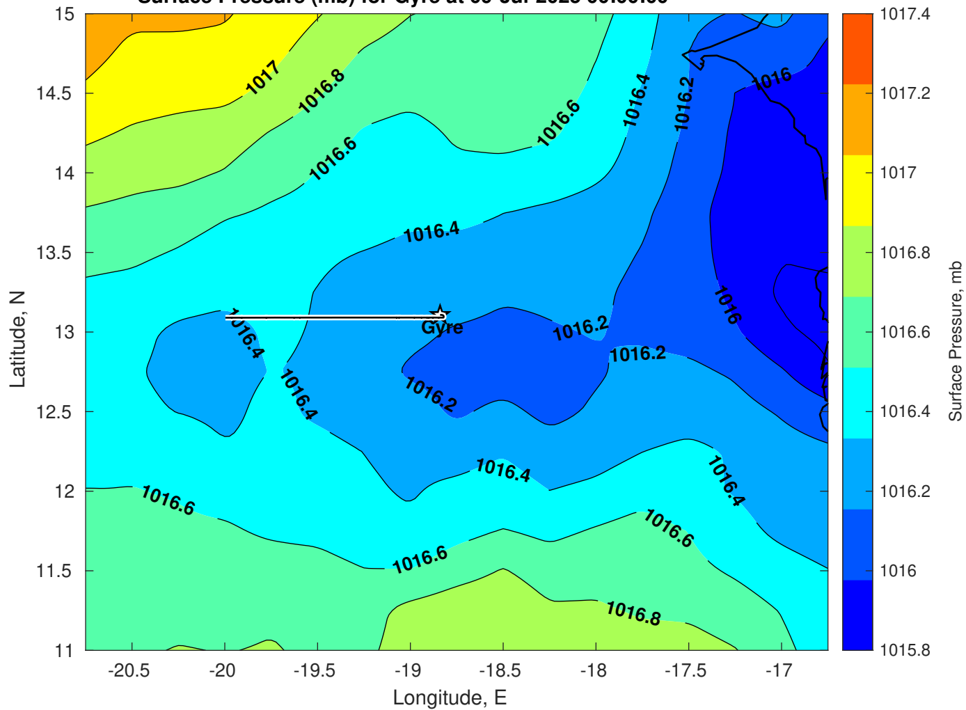
Surface Pressure (mb) for Gyre at 09-Jul-2025 00:00:00
