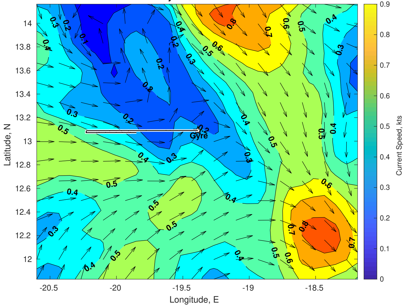
Surface Currents for Gyre at 08-Jul-2025 00:00:00
