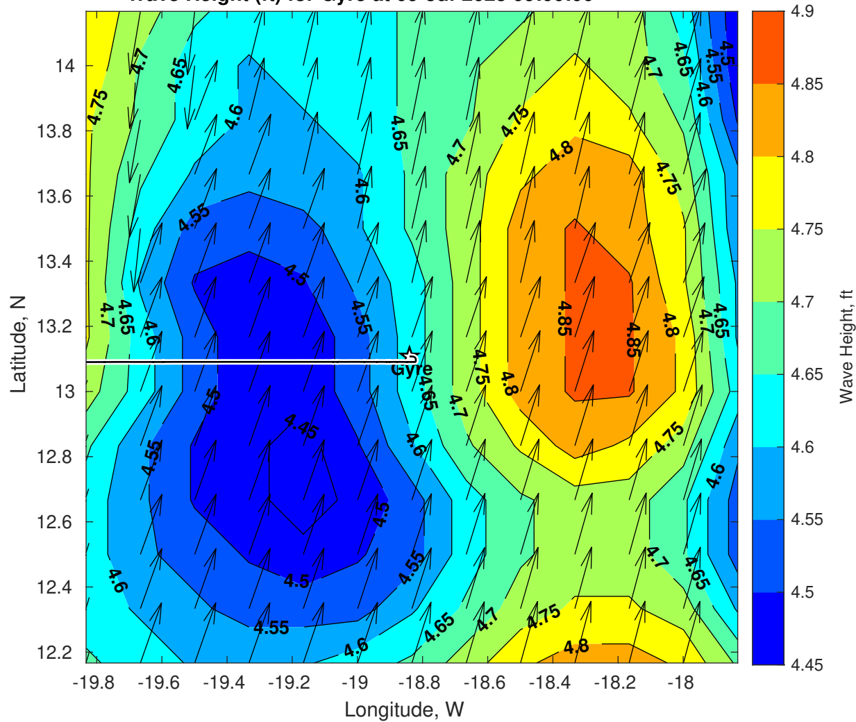
Wave Height (ft) for Gyre at 09-Jul-2025 09:00:00
