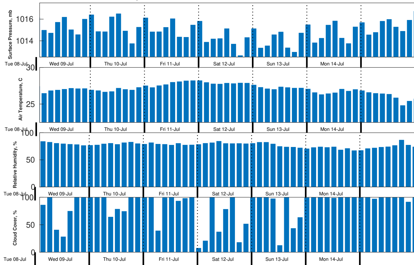
Met Forecast for Gyre from 08-Jul-2025 23:00:00 to 15-Jul-2025 23:00:00
