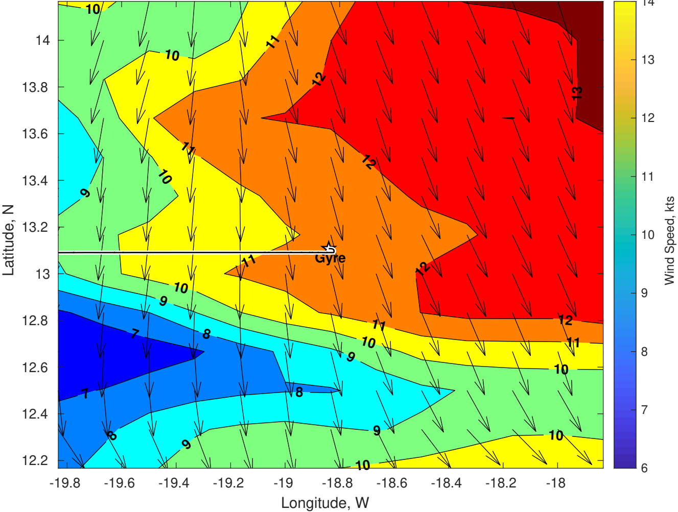
Winds (kts) for Gyre at 09-Jul-2025 09:00:00
