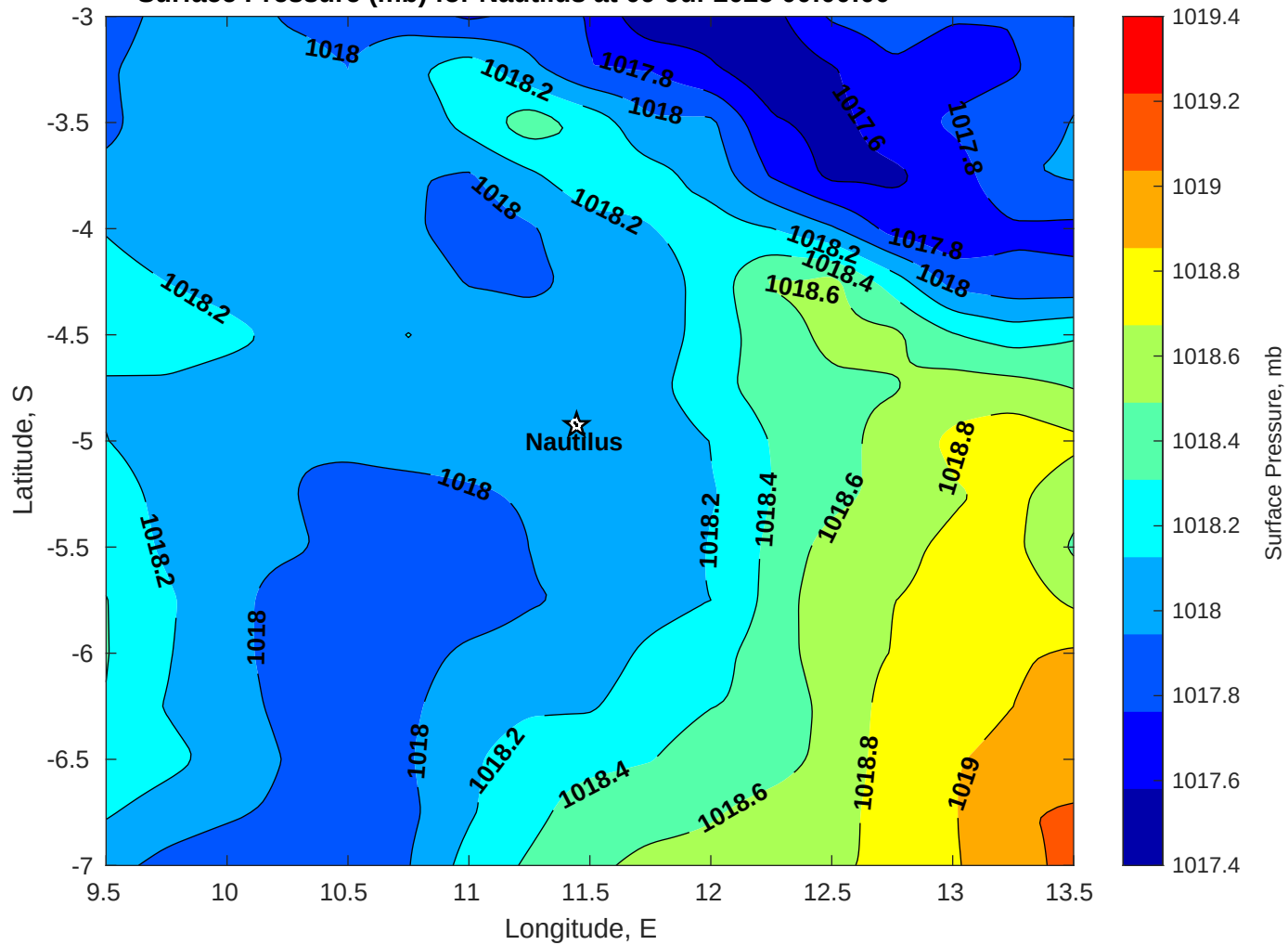
Surface Pressure (mb) for Nautilus at 09-Jul-2025 00:00:00
