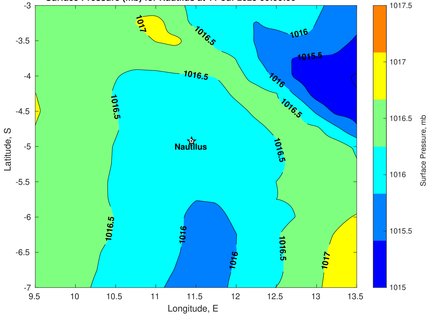
Surface Pressure (mb) for Nautilus at 11-Jul-2025 00:00:00
