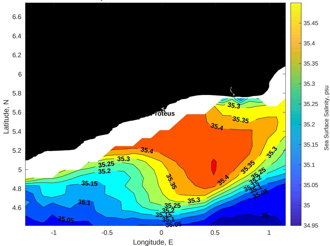
Surface Salinity for Proteus at 08-Jul-2025 00:00:00
