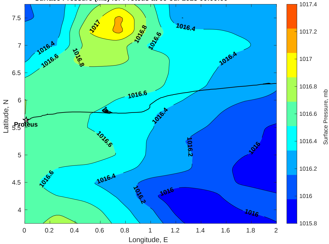
Surface Pressure (mb) for Proteus at 09-Jul-2025 00:00:00
