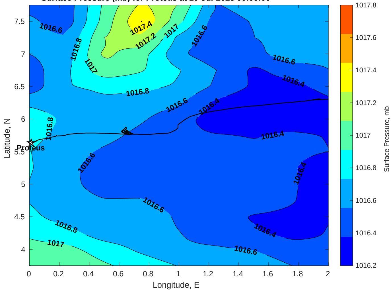
Surface Pressure (mb) for Proteus at 10-Jul-2025 00:00:00
