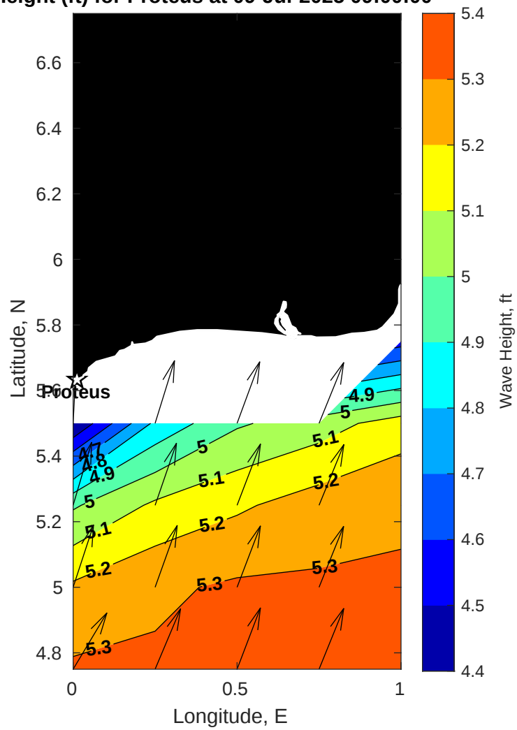
Wave Height (ft) for Proteus at 09-Jul-2025 09:00:00
