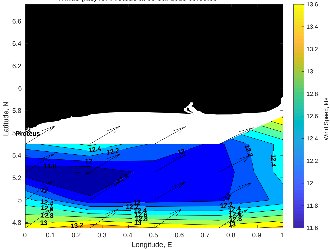
Winds (kts) for Proteus at 09-Jul-2025 09:00:00
