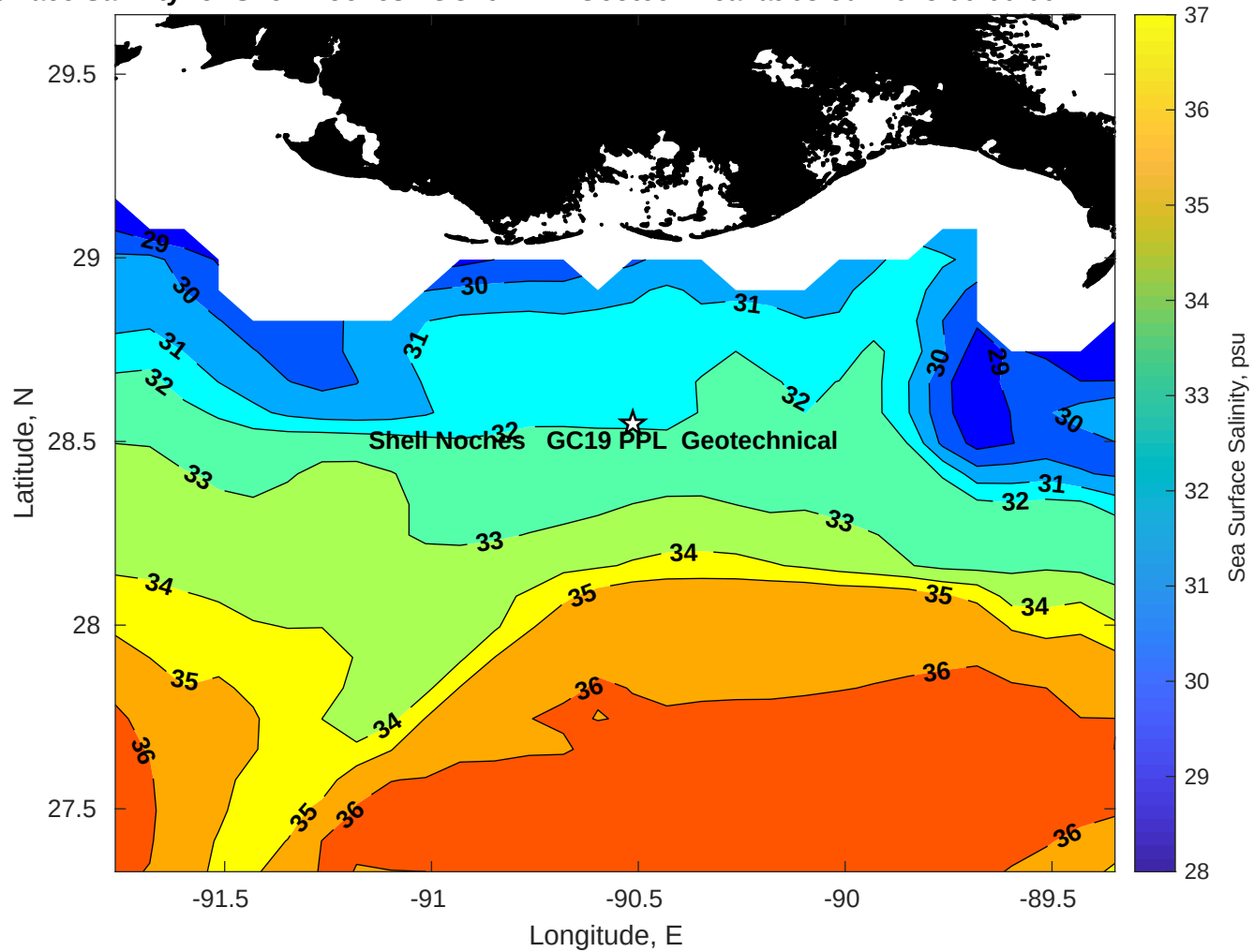
Surface Salinity for Shell Noches GC19 PPL Geotechnical at 08-Jul-2025 00:00:00
