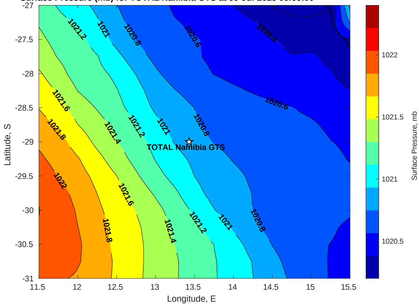
Surface Pressure (mb) for TOTAL Namibia GTS at 09-Jul-2025 00:00:00
