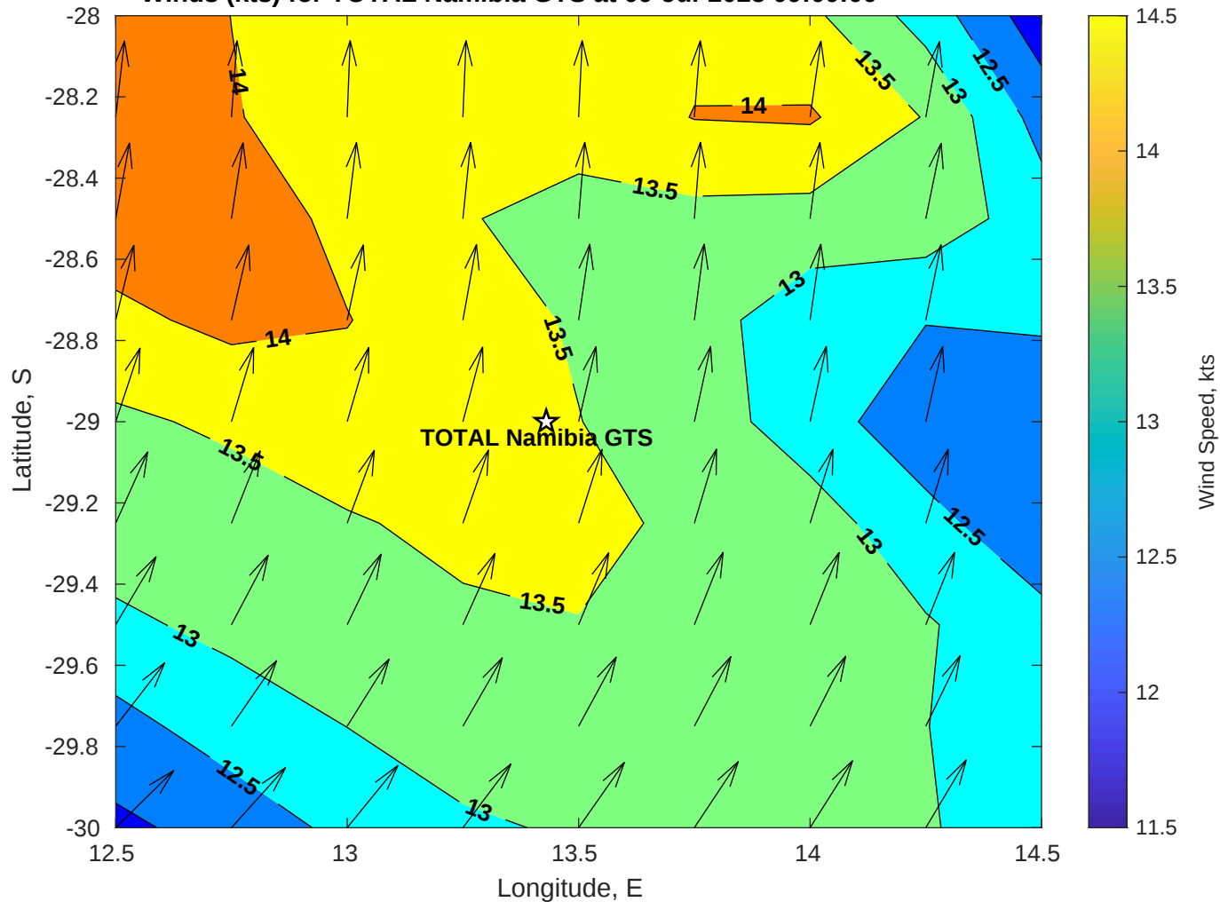
Winds (kts) for TOTAL Namibia GTS at 09-Jul-2025 09:00:00
