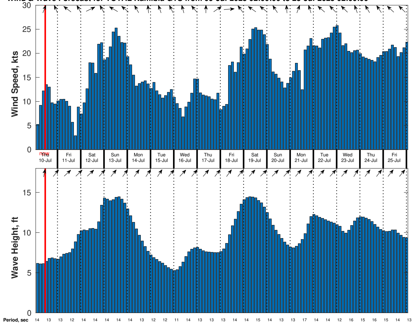
Wind & Wave Forecast for TOTAL Namibia GTS from 09-Jul-2025 02:00:00 to 25-Jul-2025 02:00:00
