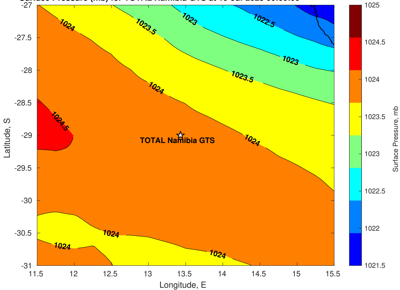
Surface Pressure (mb) for TOTAL Namibia GTS at 10-Jul-2025 00:00:00
