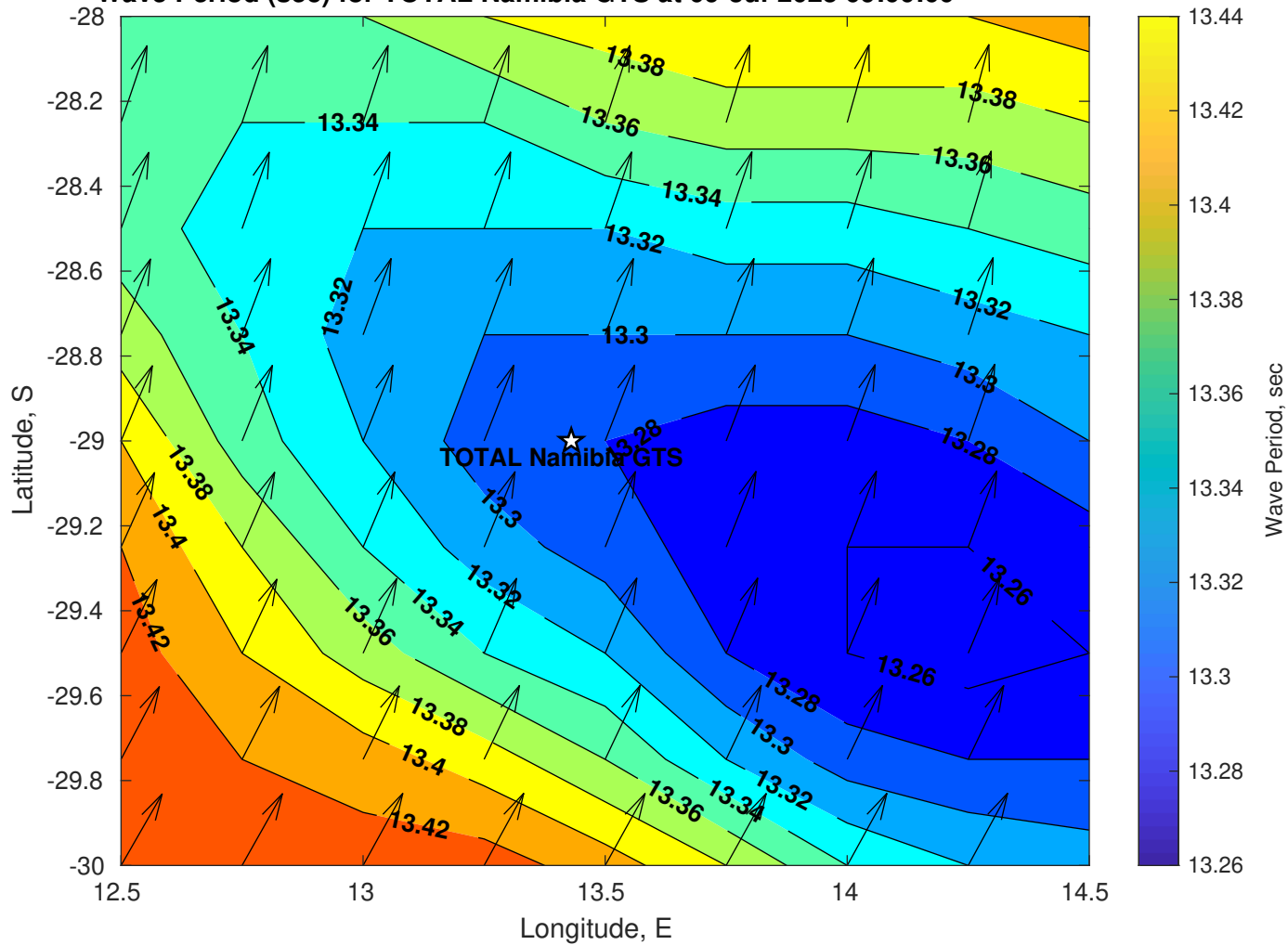
Wave Period (sec) for TOTAL Namibia GTS at 09-Jul-2025 09:00:00
