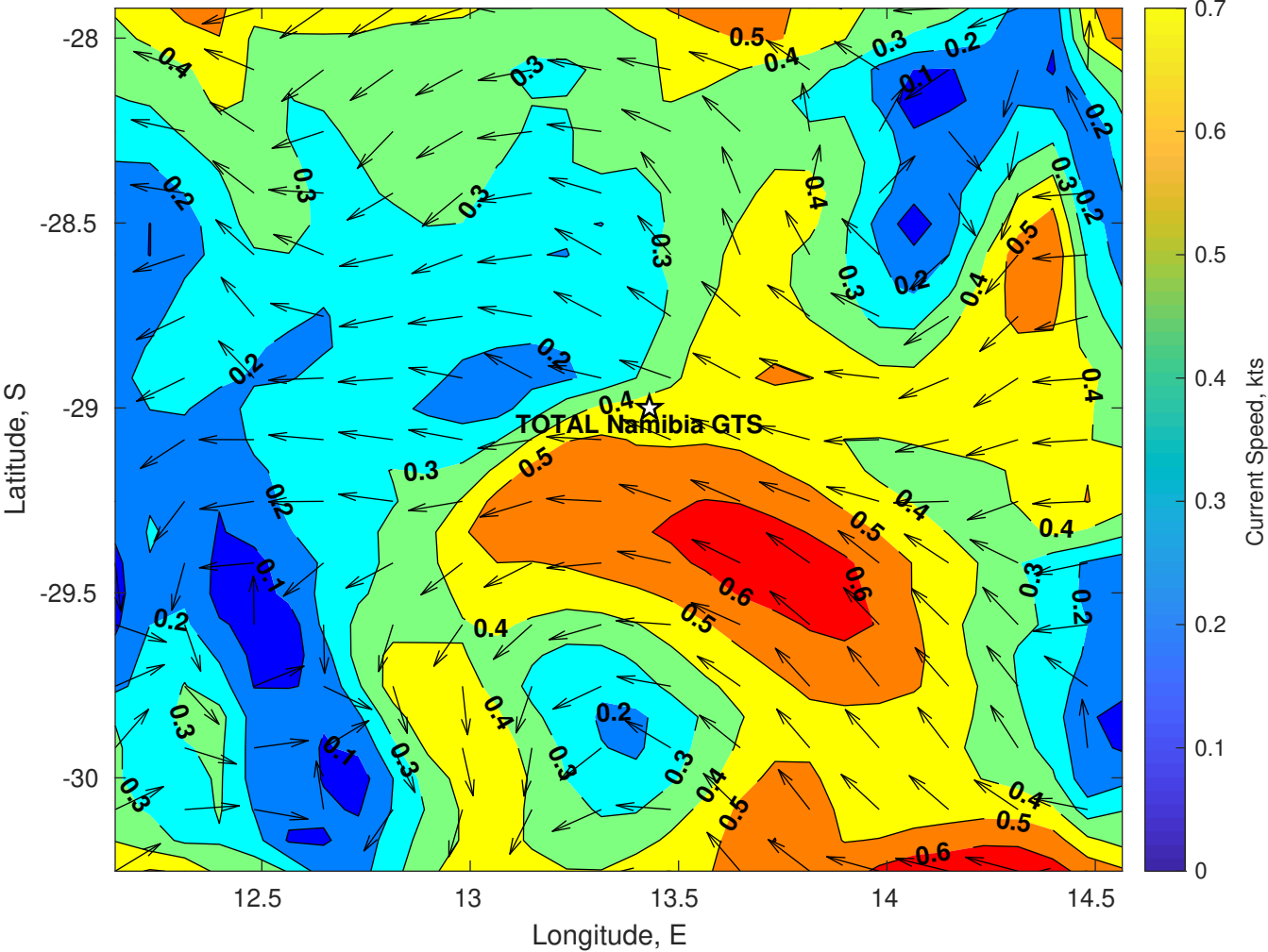
Surface Currents for TOTAL Namibia GTS at 08-Jul-2025 00:00:00
