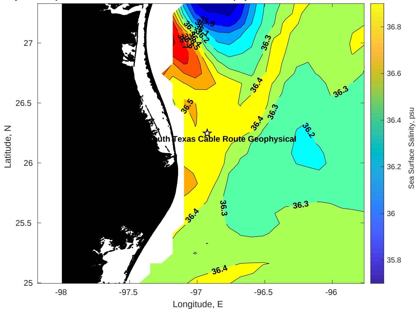
Surface Salinity for Tampnet P2378 South Texas Cable Route Geophysical at 08-Jul-2025 00:00:00
