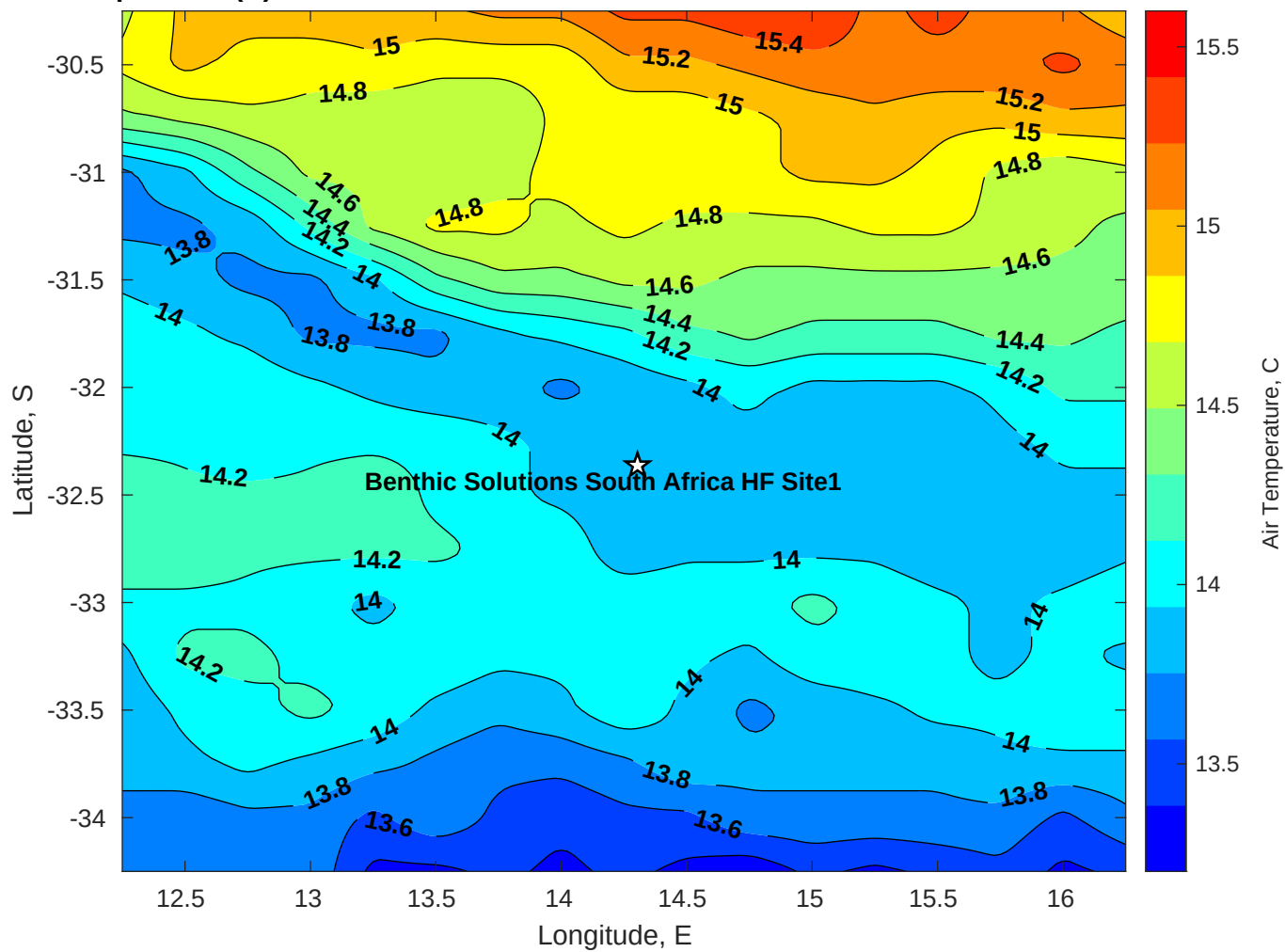
Air Temperature (C) for Benthic Solutions South Africa HF Site1 at 10-Jul-2025
