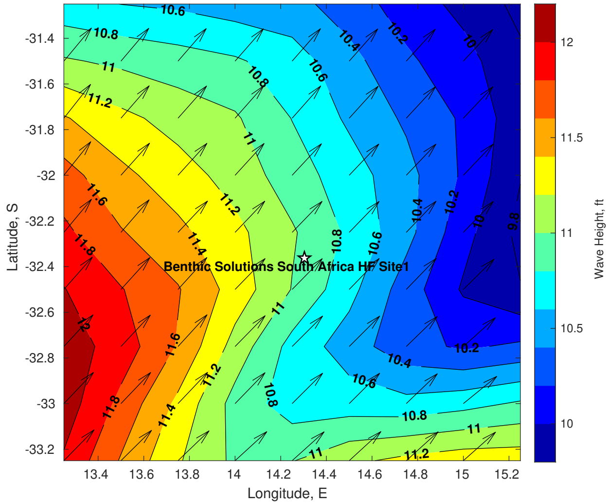
Wave Height (ft) for Benthic Solutions South Africa HF Site1 at 10-Jul-2025 09:00:00
