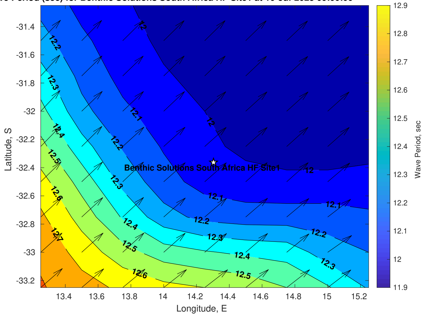
Wave Period (sec) for Benthic Solutions South Africa HF Site1 at 10-Jul-2025 09:00:00
