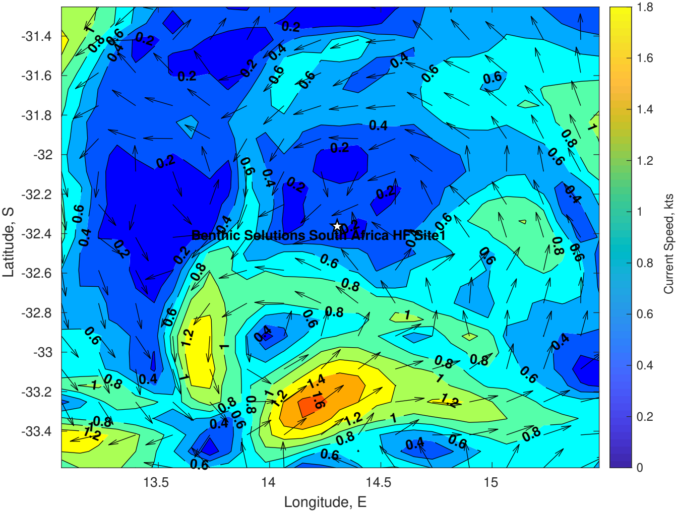
Surface Currents for Benthic Solutions South Africa HF Site1 at 09-Jul-2025 00:00:00
