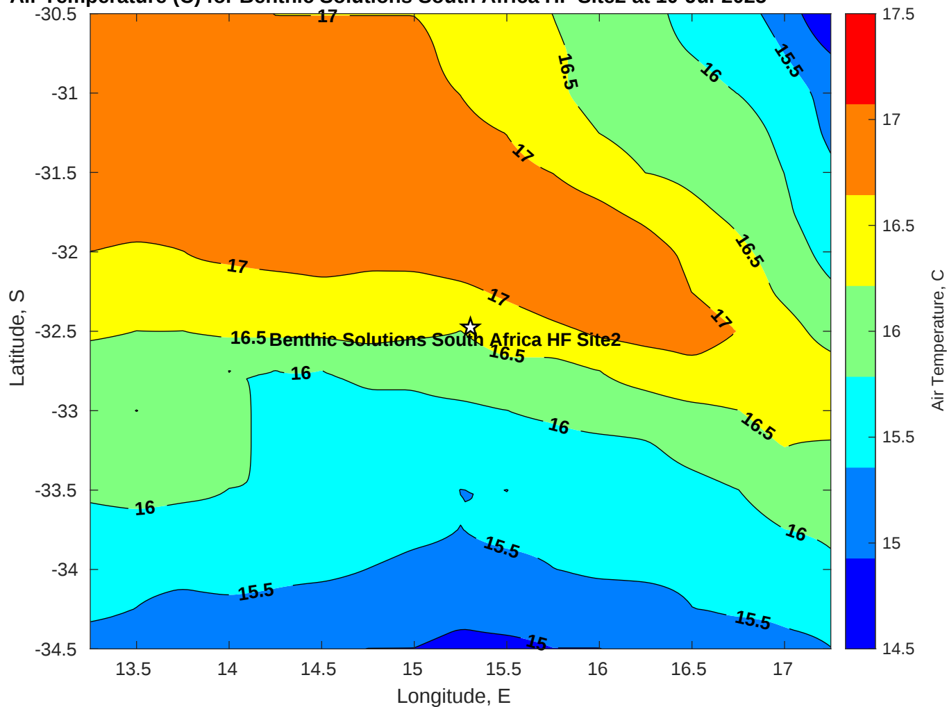
Air Temperature (C) for Benthic Solutions South Africa HF Site2 at 10-Jul-2025
