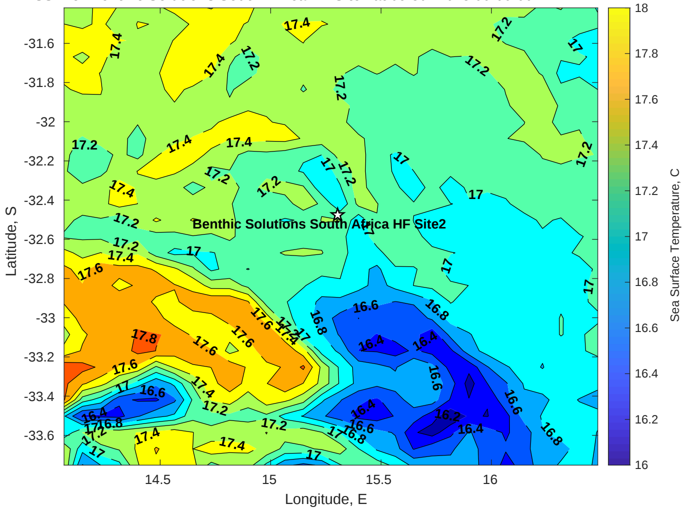
SST for Benthic Solutions South Africa HF Site2 at 09-Jul-2025 00:00:00
