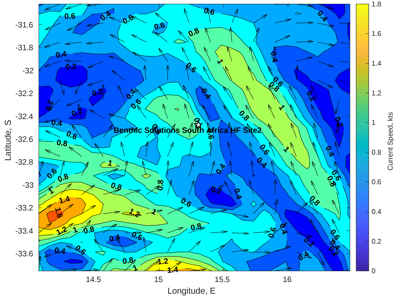
Surface Currents for Benthic Solutions South Africa HF Site2 at 09-Jul-2025 00:00:00
