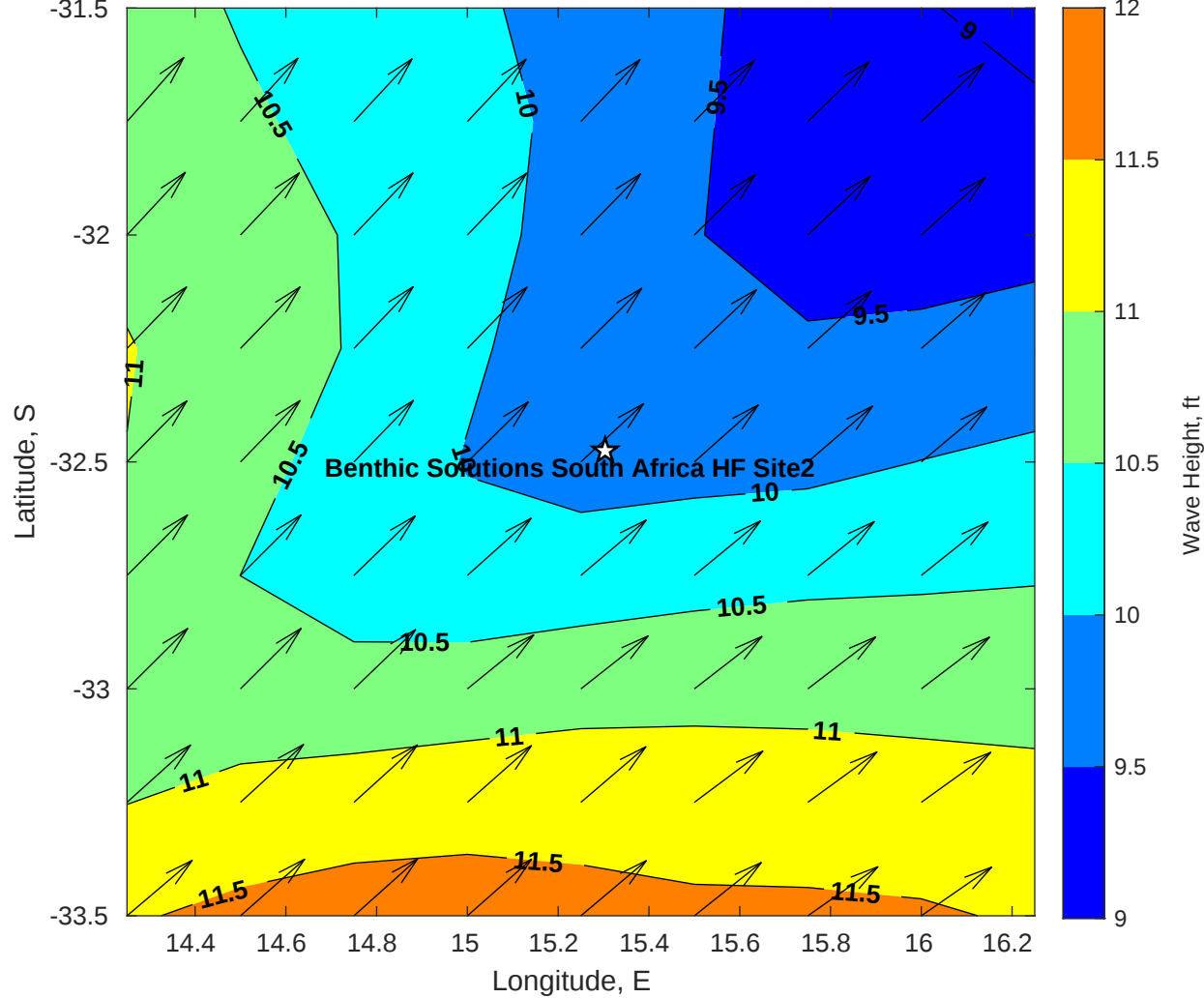
Wave Height (ft) for Benthic Solutions South Africa HF Site2 at 10-Jul-2025 09:00:00
