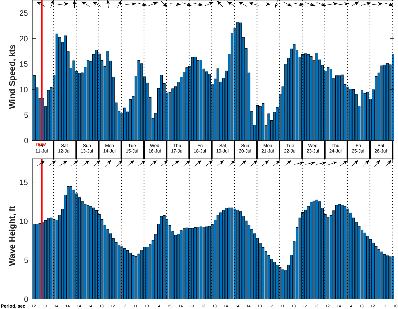
Wind & Wave Forecast for Benthic Solutions South Africa HF Site2 from 10-Jul-2025 02:00:00 to 26-Jul-2025 02:00:00
