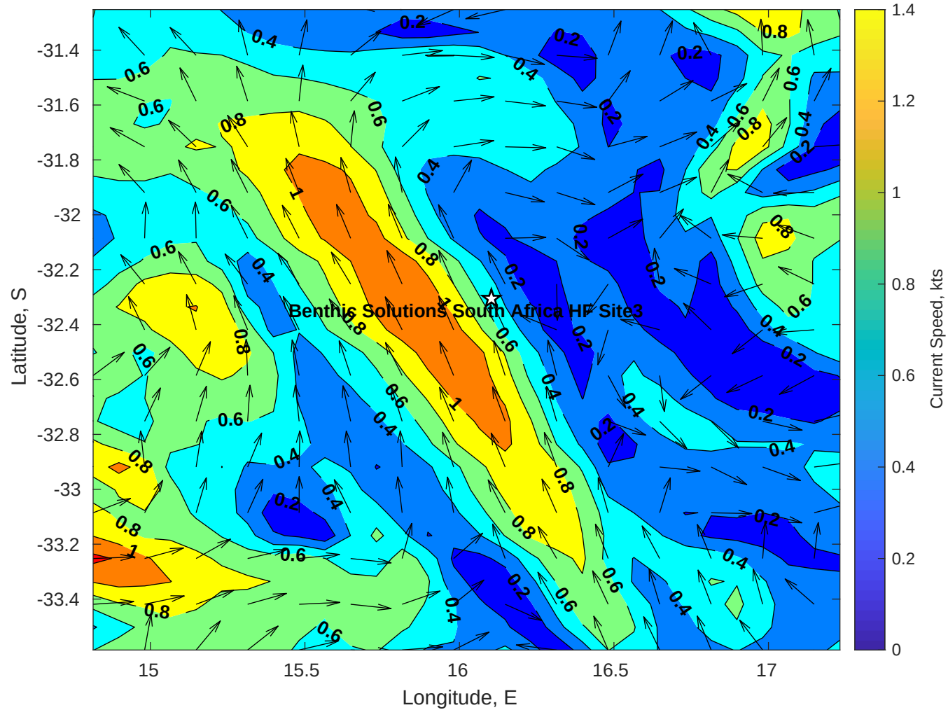
Surface Currents for Benthic Solutions South Africa HF Site3 at 09-Jul-2025 00:00:00
