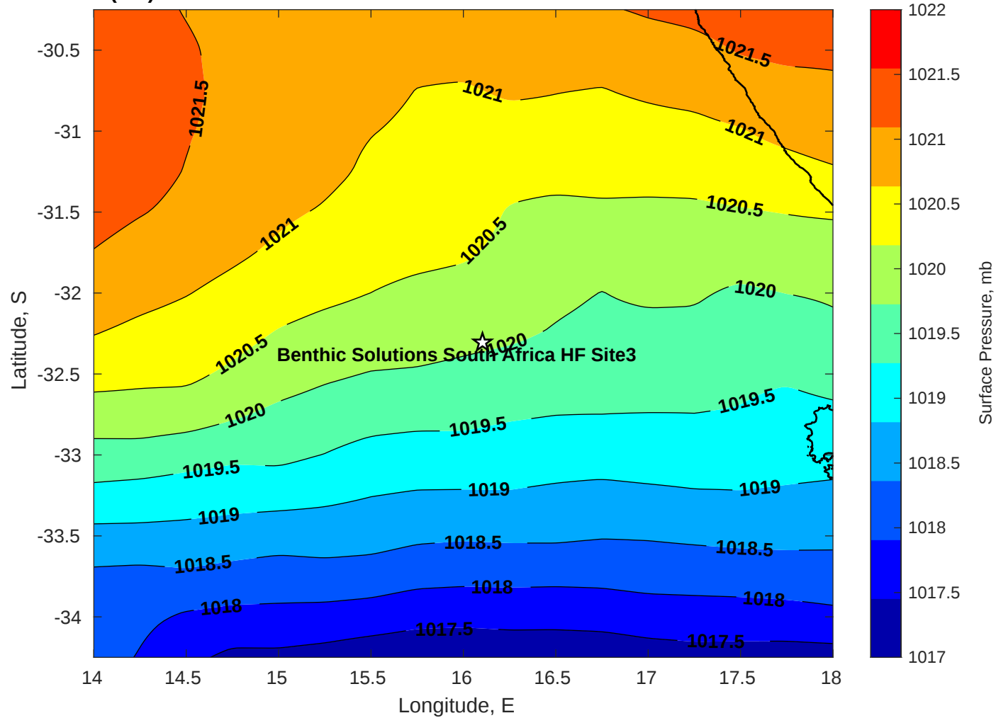
Surface Pressure (mb) for Benthic Solutions South Africa HF Site3 at 11-Jul-2025 00:00:00
