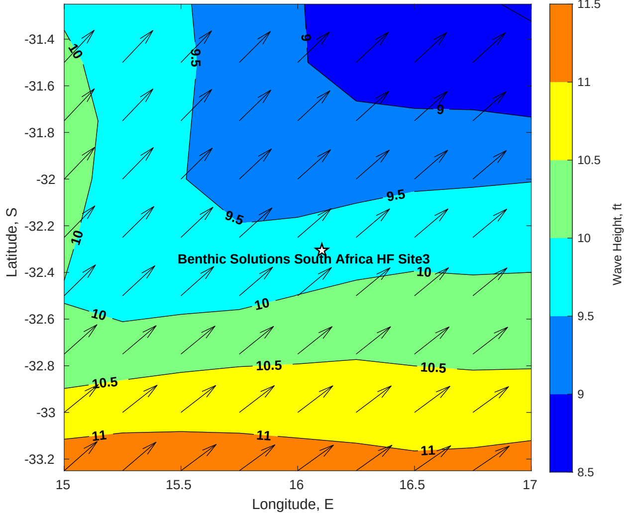
Wave Height (ft) for Benthic Solutions South Africa HF Site3 at 10-Jul-2025 09:00:00
