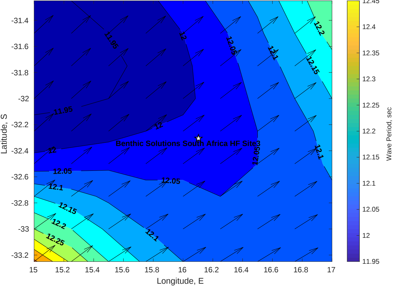
Wave Period (sec) for Benthic Solutions South Africa HF Site3 at 10-Jul-2025 09:00:00
