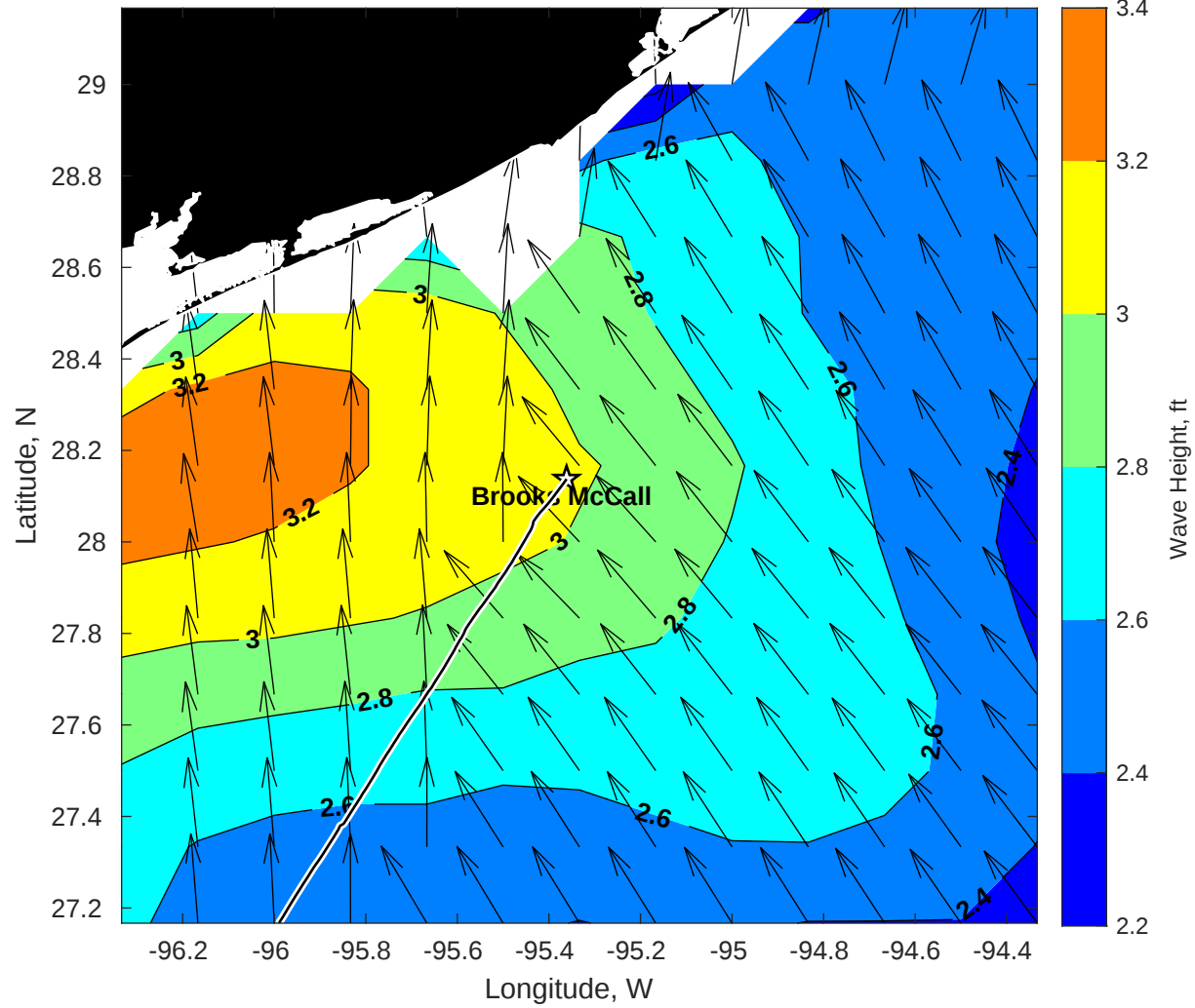
Wave Height (ft) for Brooks McCall at 10-Jul-2025 09:00:00
