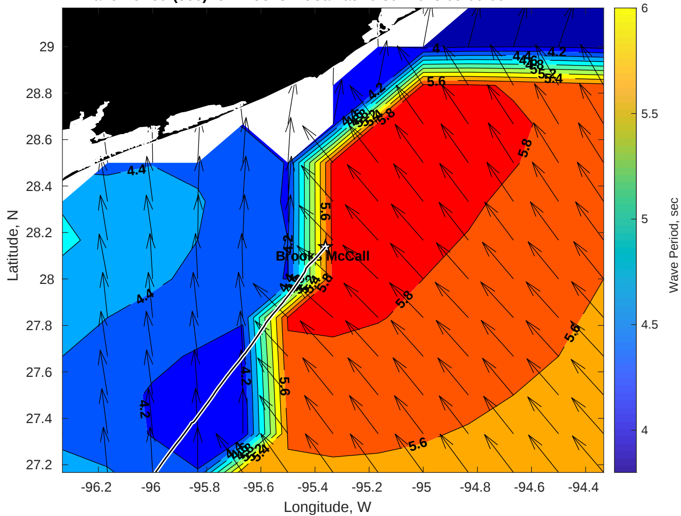
Wave Period (sec) for Brooks McCall at 10-Jul-2025 09:00:00
