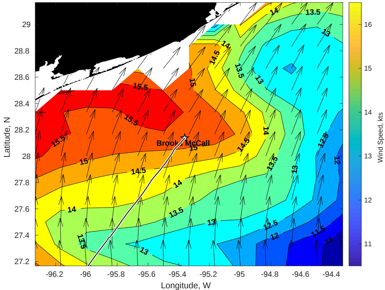
Winds (kts) for Brooks McCall at 10-Jul-2025 09:00:00
