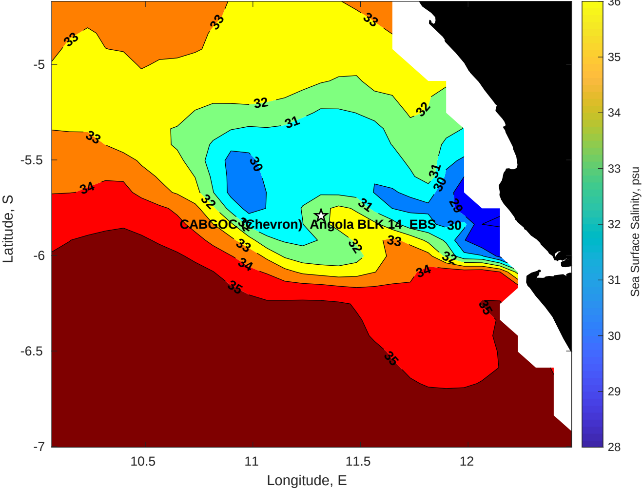
Surface Salinity for CABGOC (Chevron) Angola BLK 14 EBS at 09-Jul-2025 00:00:00
