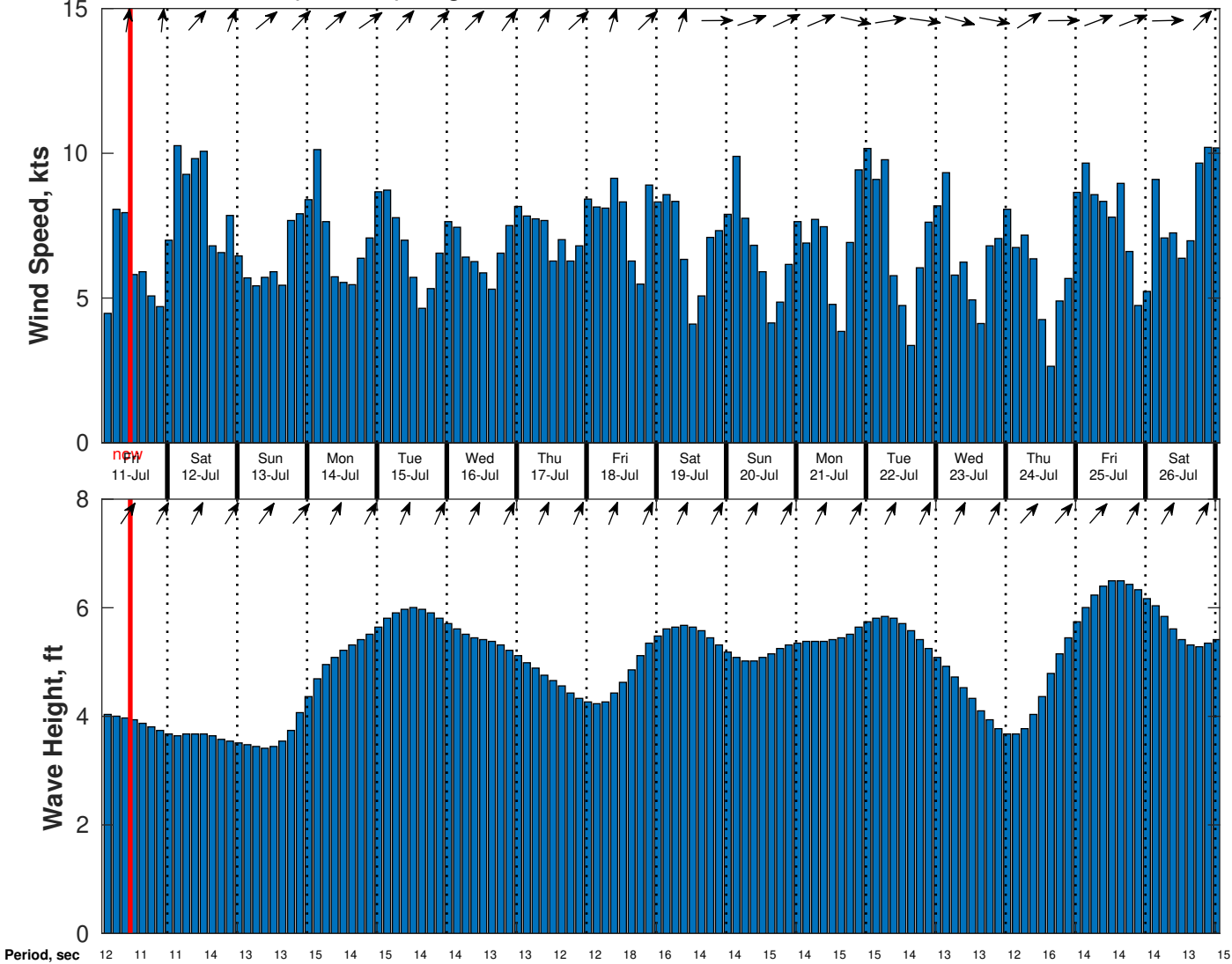
Wind & Wave Forecast for CABGOC (Chevron) Angola BLK 14 EBS from 10-Jul-2025 02:00:00 to 26-Jul-2025 02:00:00
