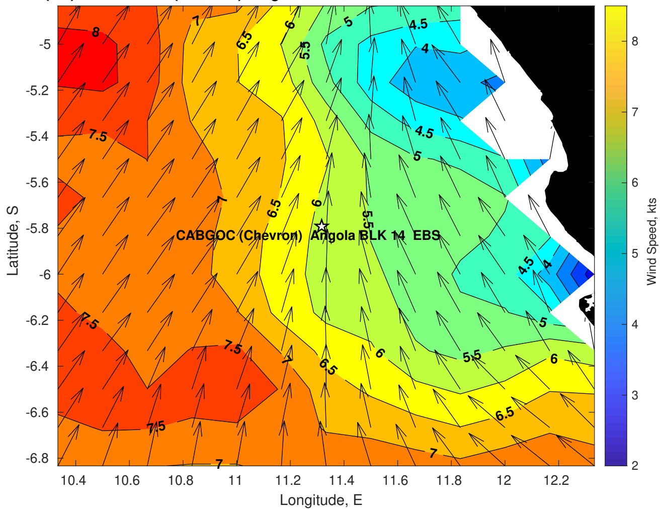
Winds (kts) for CABGOC (Chevron) Angola BLK 14 EBS at 10-Jul-2025 09:00:00
