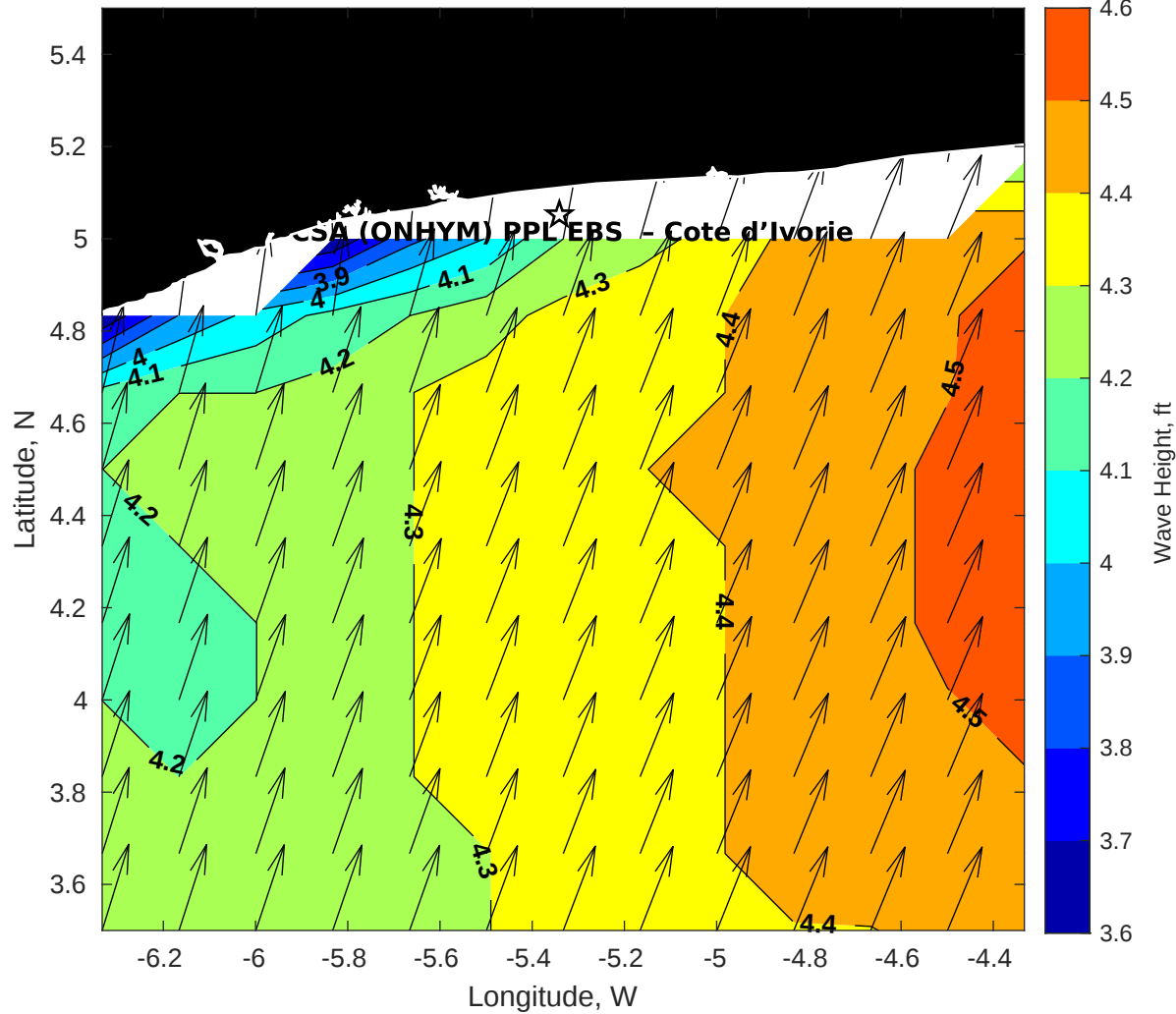
Wave Height (ft) for CSA (ONHYM) PPL EBS - Cote d'Ivoire at 10-Jul-2025 09:00:00
