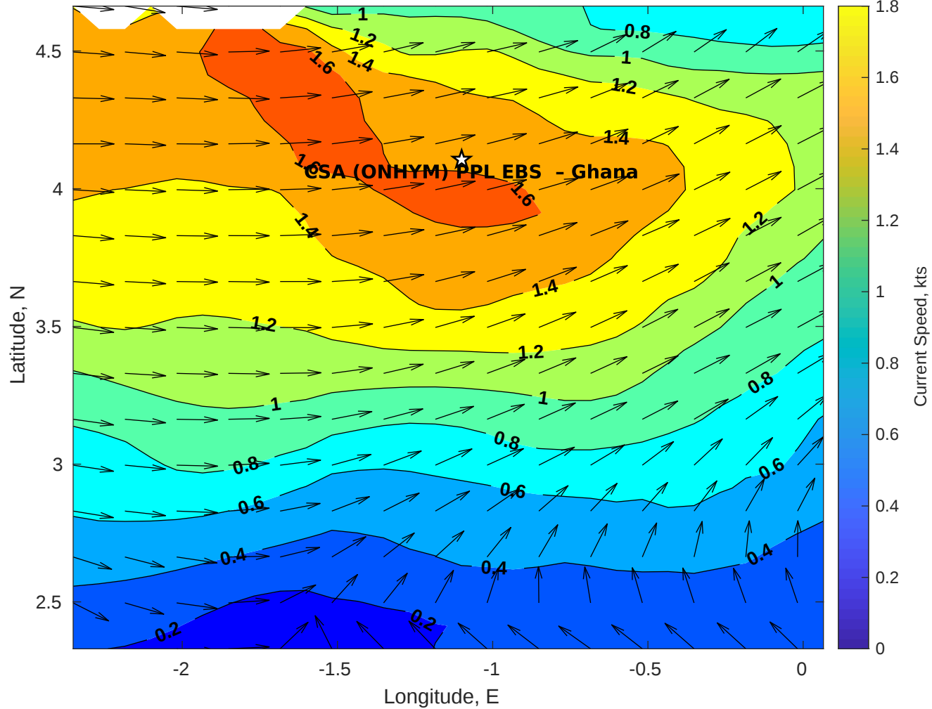
Surface Currents for CSA (ONHYM) PPL EBS - Ghana at 09-Jul-2025 00:00:00
