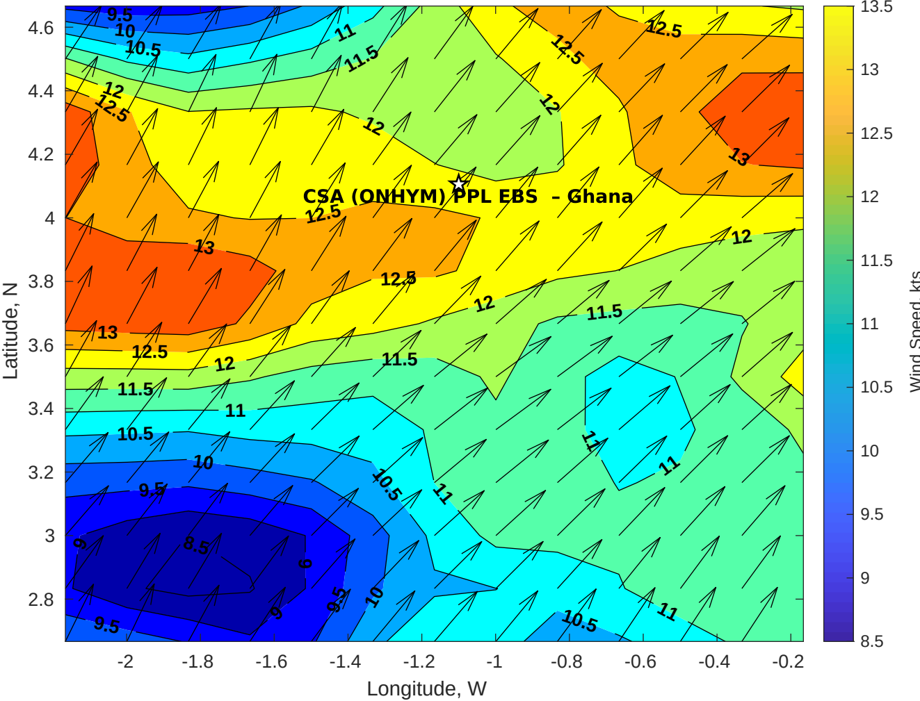
Winds (kts) for CSA (ONHYM) PPL EBS - Ghana at 10-Jul-2025 09:00:00
