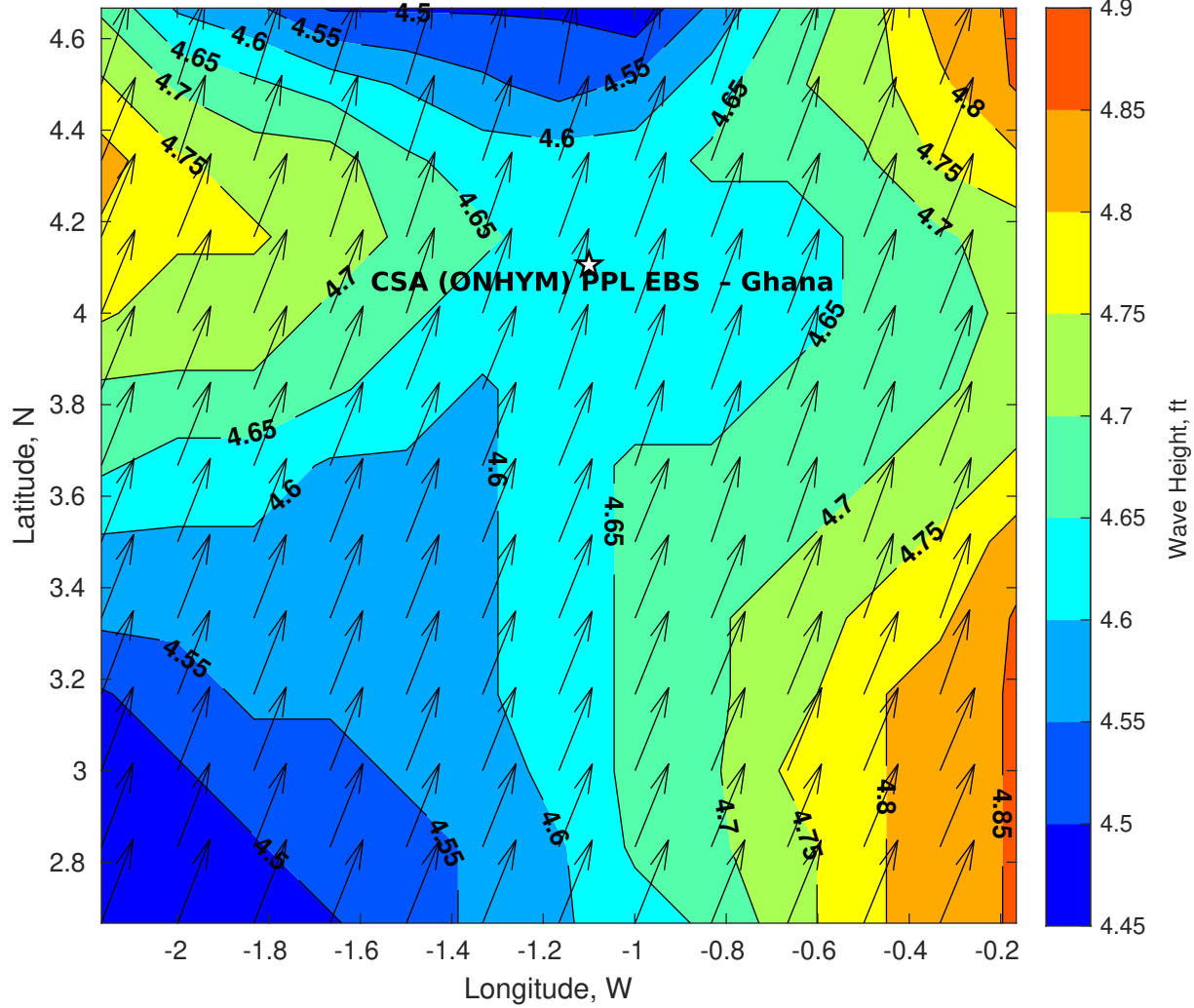
Wave Height (ft) for CSA (ONHYM) PPL EBS - Ghana at 10-Jul-2025 09:00:00
