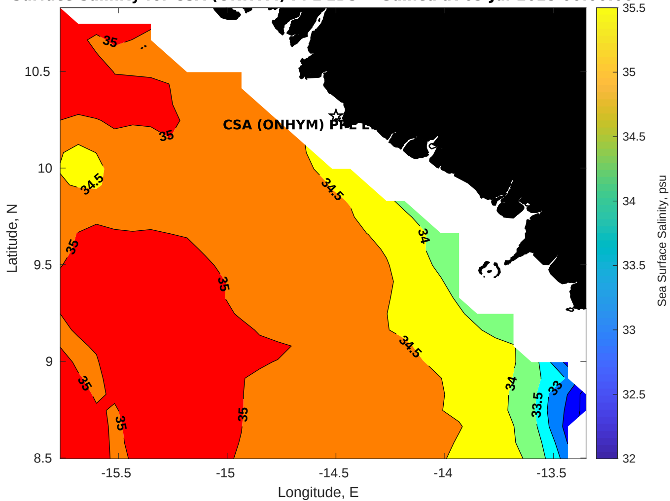
Surface Salinity for CSA (ONHYM) PPL EBS - Guinea at 09-Jul-2025 00:00:00
