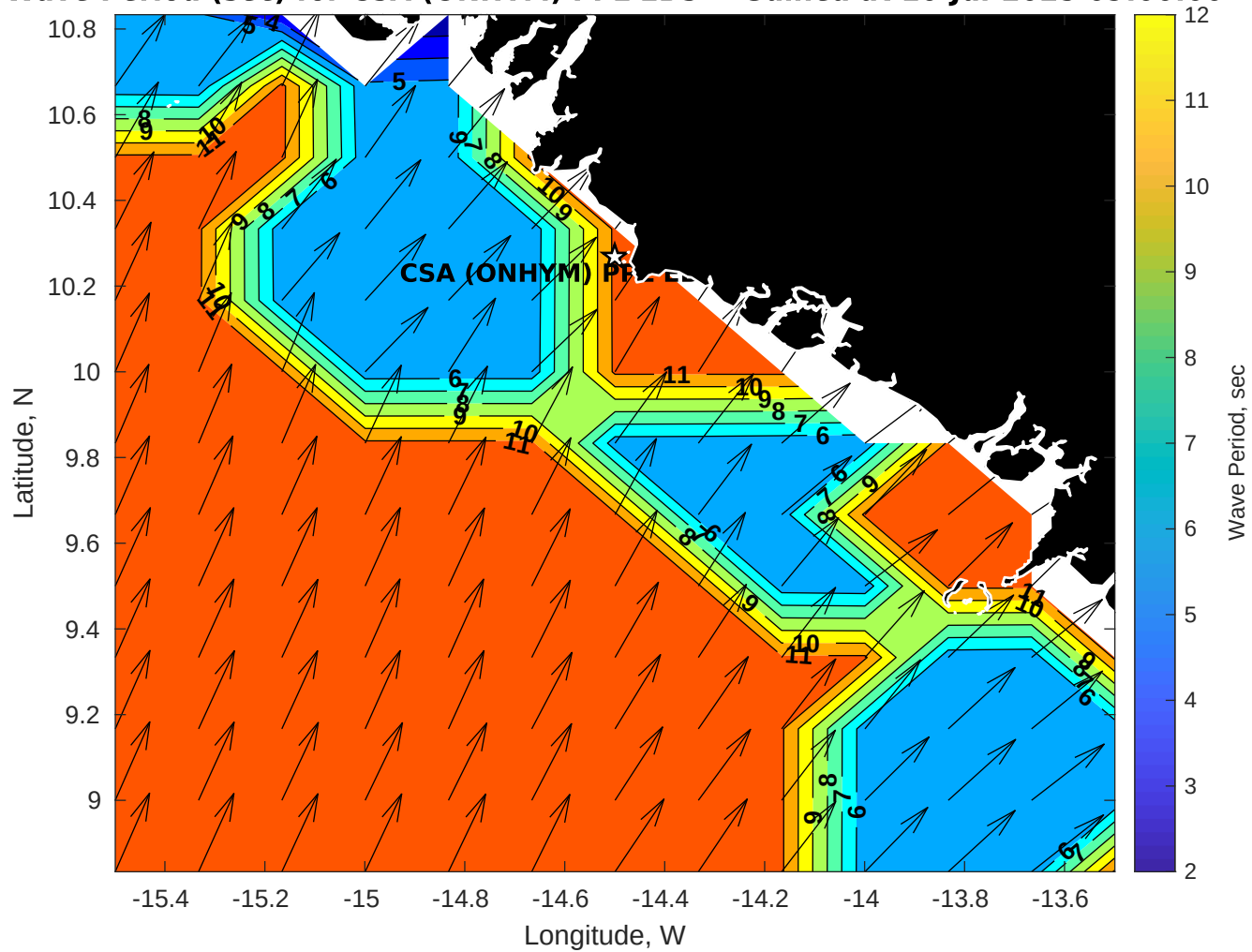
Wave Period (sec) for CSA (ONHYM) PPL EBS - Guinea at 10-Jul-2025 09:00:00
